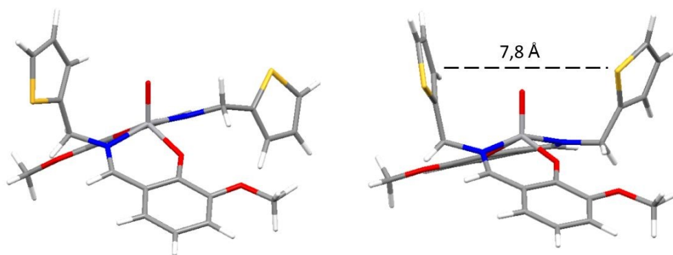
Figure 3. Optimized geometries of [\text{VO}(\text{oVATPNH}_2)_2] taking different geometry as starting points. Left: thiophene rings in trans conformation. Right: thiophene rings in cis conformation. The distance between the thiophene rings is shown for the latter.
