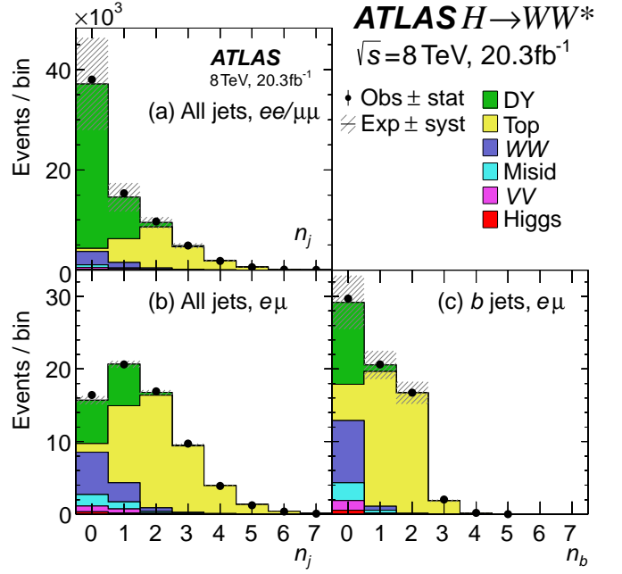
FIG. 6. Jet multiplicity distributions for all jets ( n_j ) and b -tagged jets ( n_b ). The plots are made after applying the preselection criteria common to all n_j categories (see Table IV). See Fig. 5 for plotting details.
