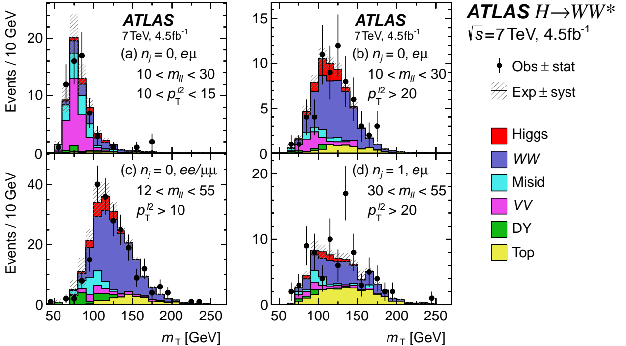
FIG. 34. Post-fit transverse mass distributions in the n_j \leq 1 categories in the 7 TeV data analysis, for specific m_{\ell\ell} and p_T^{\ell\ell} ranges. The plots are made after applying all the selection requirements (see Sec. IV E). See Figs. 5 and 29 for plotting details.
