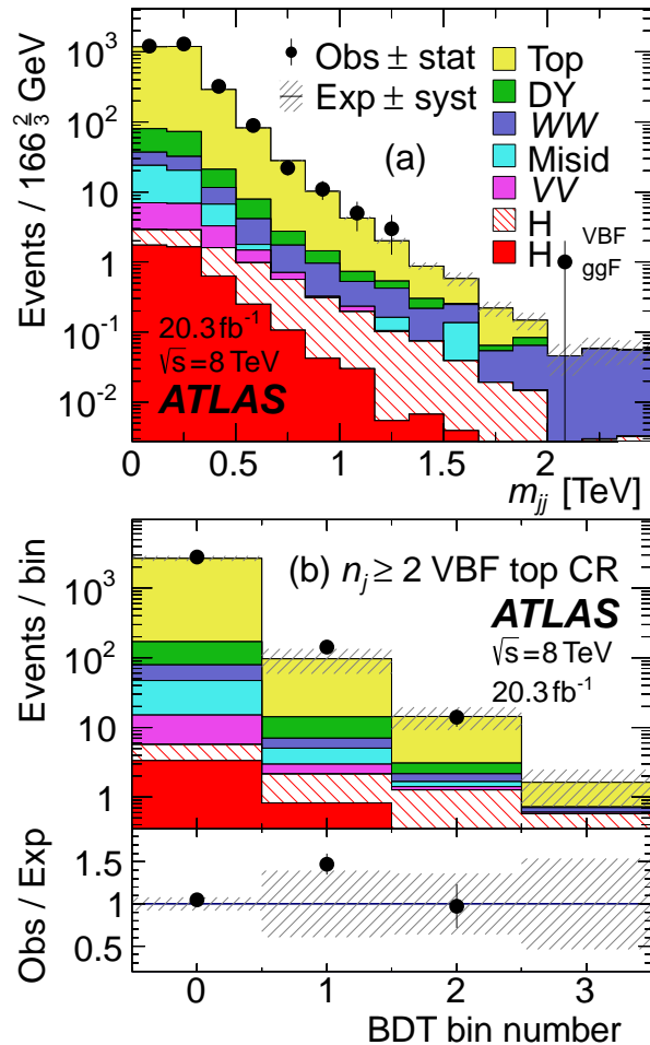
FIG. 22. Top-quark control region (CR) distributions in the VBF-enriched n_j \geq 2 category for: (a) m_{jj} and (b) BDT output. For the plot in (b) the shaded band in the ratio shows the uncertainty on the normalization of each bin. No events are observed in bin 3. See Fig. 5 for plotting details.
