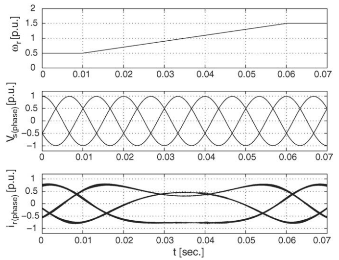
Fig. 7. Speed change.
