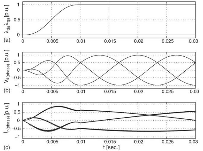
Fig. 4. System turn-on: (a) (–) stator fluxes; (– · –) stator flux references, (b) stator phase voltages and (c) rotor phase currents.
