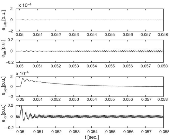
Fig. 6. Current and flux errors.
