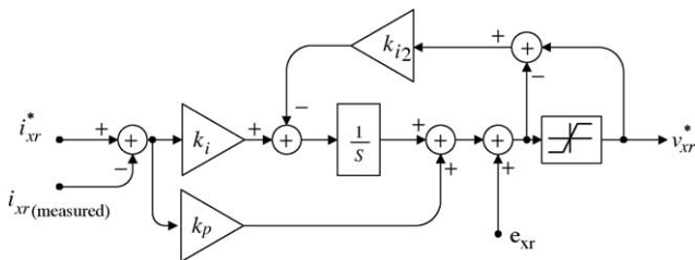
Fig. 2. PI with anti windup and feed forward compensating term.
