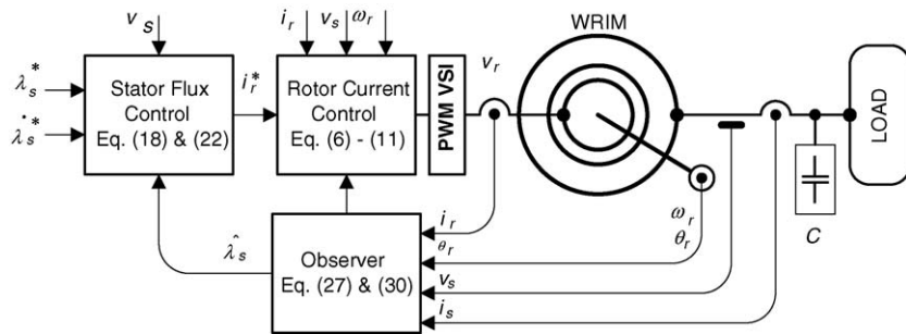
Fig. 3. Simplified block diagram.
