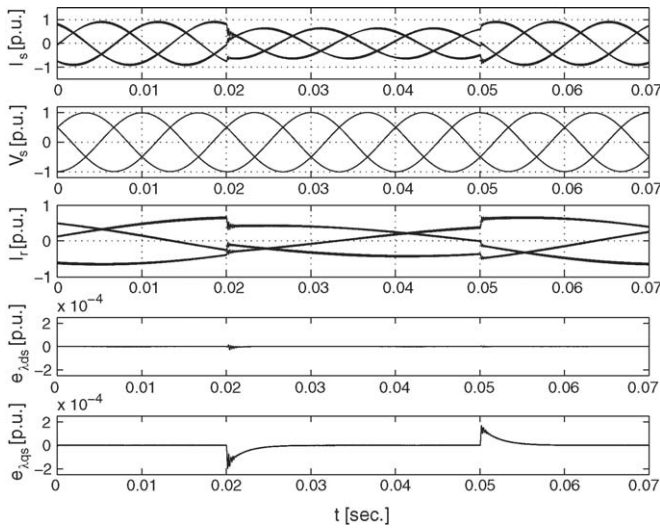
Fig. 5. Load change.
