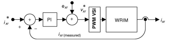
Fig. 1. Current control loop ( x=d, q ).
