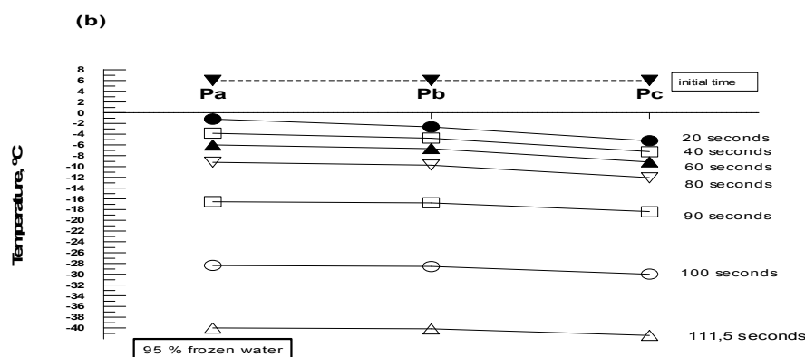
Figure 3. (a) Internal temperature gradients in 0.5 ml straw filled with spermatozoa during freezing in nitrogen vapor at -100^{\circ}\text{C} and h = 5 \text{ W}/(\text{m}^2 \text{ K}) (for meaning of Pa , Pb and Pc see Figure 1). (b) Internal temperature gradients in 0.5 ml straw filled with spermatozoa during freezing in nitrogen vapor at -100^{\circ}\text{C} and h = 15 \text{ W}/(\text{m}^2 \text{ K}) (for meaning of Pa , Pb and Pc see Figure 1).
