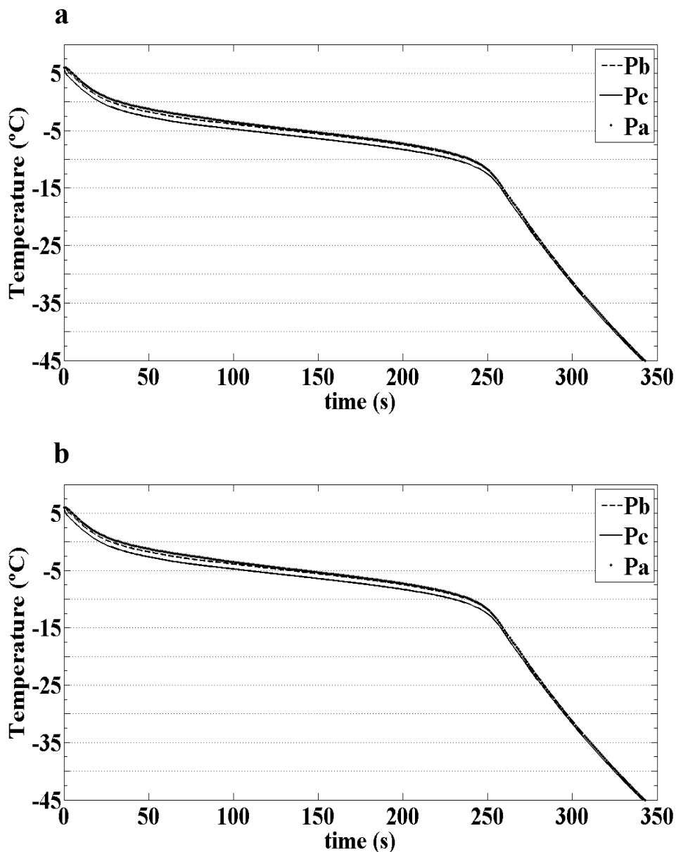
Figure 2. (a) Predicted temperature evolution at different locations in straw (see Figure 1) during cooling in nitrogen vapor at -100^\circ\text{C} and h = 5 \text{ W}/(\text{m}^2 \text{ K}) , (b) Predictive temperature evolution at different locations in straw (see Figure 1) during cooling in nitrogen vapor at -100^\circ\text{C} and h = 15 \text{ W}/(\text{m}^2 \text{ K}) (for meaning of Pa, Pb and Pc, see Figure 1).
