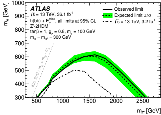
Figure 2: Exclusion contours for the Z' -2HDM scenario in the (m_{Z'}, m_A) plane for \tan\beta = 1 , g_{Z'} = 0.8 , and m_\chi = 100 GeV. The observed limits (solid line) are consistent with the expectation under the SM-only hypothesis (dashed line) within uncertainties (filled band). Observed limits from previous ATLAS results at \sqrt{s} = 13 TeV (dash-dotted line) [30] are also shown.
