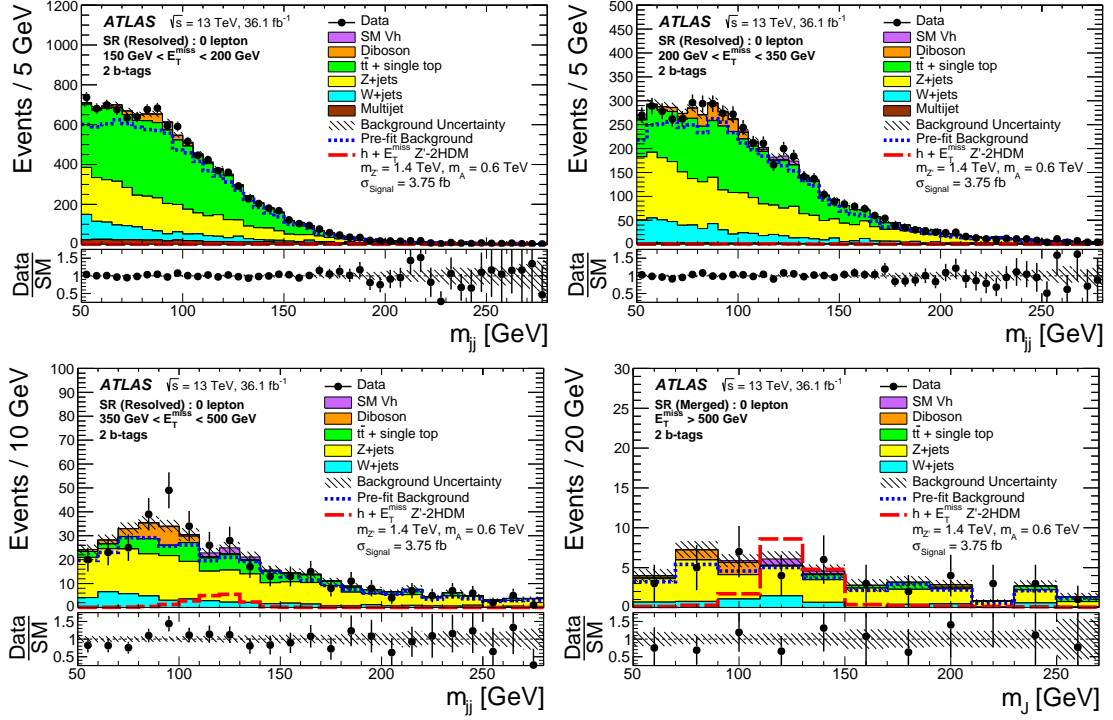
Figure 1: Distributions of the invariant mass of the Higgs boson candidates m_h = m_{jj}, m_J with two b -tags in the SR for the four E_T^{\text{miss}} categories that are used as inputs to the fit. The upper panels show a comparison of data to the SM expectation before (dashed lines) and after the fit (solid histograms) with no signal included. The lower panels display the ratio of data to SM expectations after the fit, with its systematic uncertainty considering correlations between individual contributions indicated by the hatched band. The expected signal from a representative Z' -2HDM model is also shown (long-dashed line).
