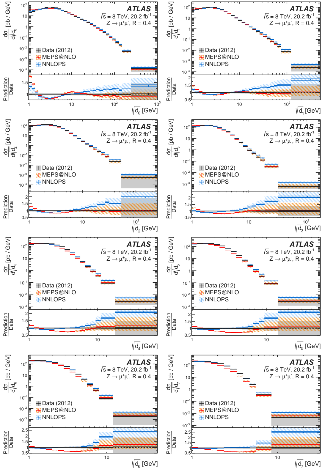
Figure 7: Charged-only distributions for the eight leading splitting scales in the muon channel using the jet-radius parameter R = 0.4 . The size of the error bars reflects the statistical uncertainty, while the combined statistical and systematic uncertainty is indicated by the grey band. Theoretical predictions from SHERPA with NLO multijet merging (“MEPS@NLO”) and from POWHEG+PYTHIA 8 with NNLO matching (“NNLOPS”) are displayed.
