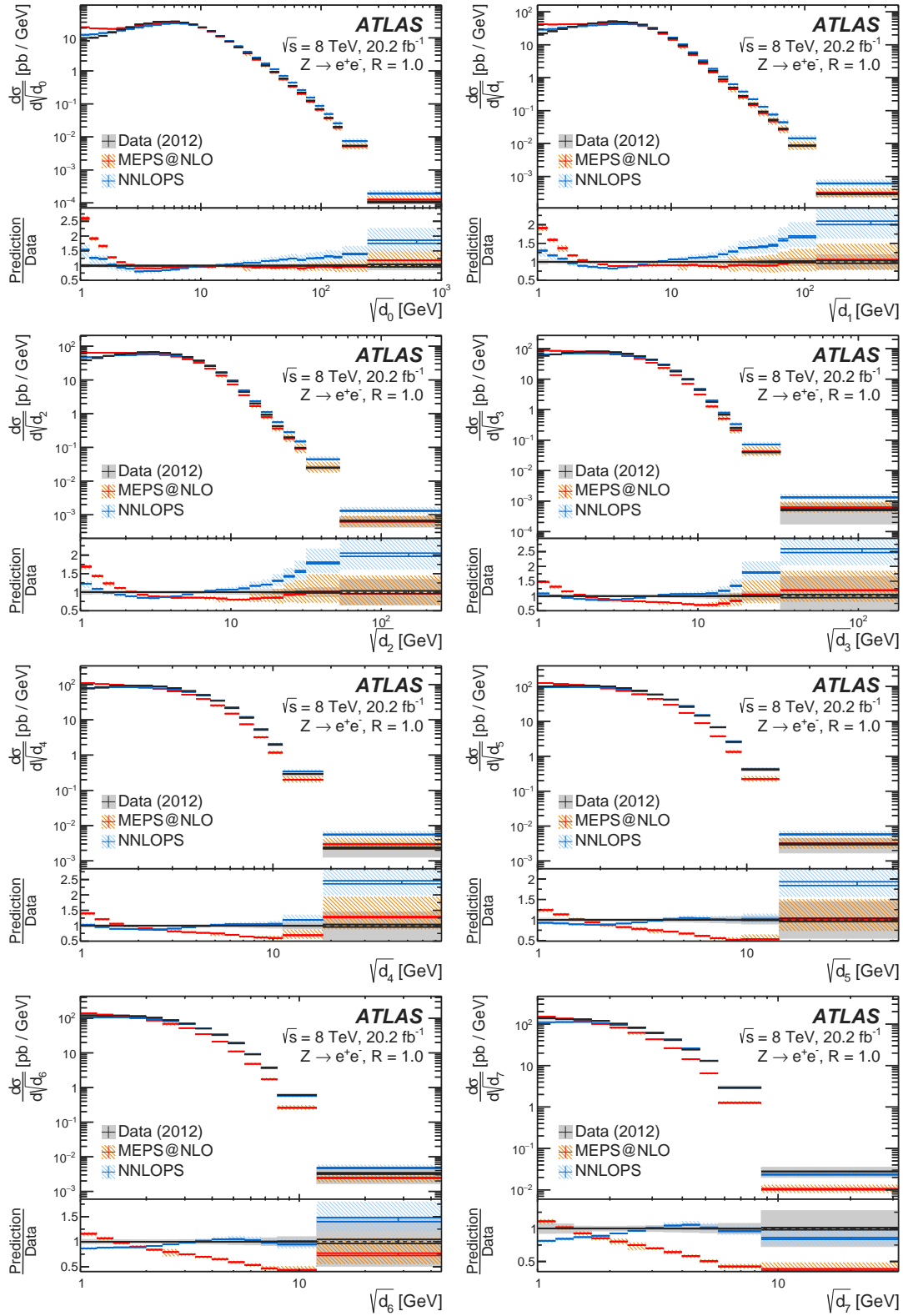
Figure 6: Charged-only distributions for the eight leading splitting scales in the electron channel using the jet-radius parameter R = 1.0 . The size of the error bars reflects the statistical uncertainty, while the combined statistical and systematic uncertainty is indicated by the grey band. Theoretical predictions from SHERPA with NLO multijet merging (“MEPS@NLO”) and from PowHEG+PYTHIA 8 with NNLO matching (“NNLOPS”) are displayed.
