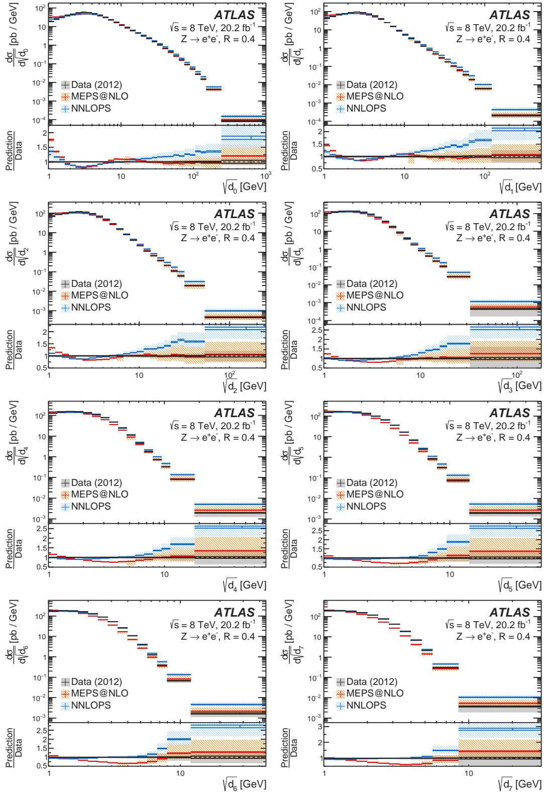
Figure 4: Charged-only distributions for the eight leading splitting scales in the electron channel using the jet-radius parameter R = 0.4 . The size of the error bars reflects the statistical uncertainty, while the combined statistical and systematic uncertainty is indicated by the grey band. Theoretical predictions from SHERPA with NLO multijet merging (“MEPS@NLO”) and from POWHEG+PYTHIA 8 with NNLO matching (“NNLOPS”) are displayed including error bands for the generator uncertainties.
