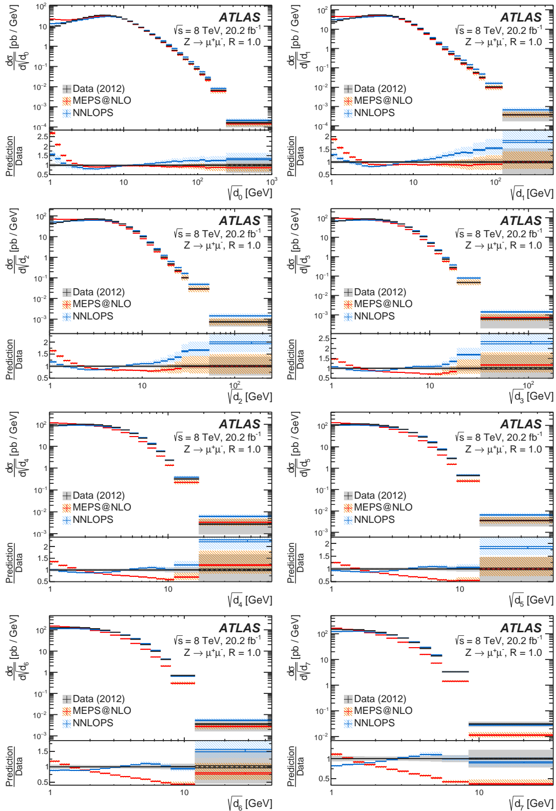
Figure 8: Charged-only distributions for the eight leading splitting scales in the muon channel using the jet-radius parameter R = 1.0 . The size of the error bars reflects the statistical uncertainty, while the combined statistical and systematic uncertainty is indicated by the grey band. Theoretical predictions from SHERPA with NLO multijet merging (“MEPS@NLO”) and from POWHEG+PYTHIA 8 with NNLO matching (“NNLOPS”) are displayed.
