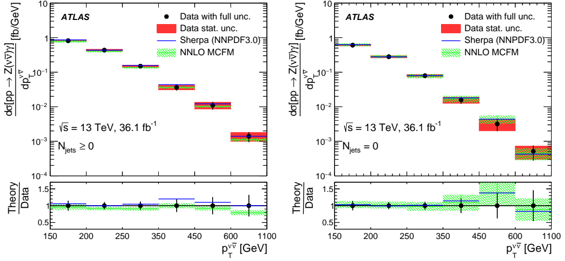
Figure 5: The measured (points with error bars) and predicted differential cross sections as a function of p_T^{v\bar{v}} for the pp \rightarrow Z(v\bar{v})\gamma process in the inclusive N_{\text{jets}} \geq 0 (left) and exclusive N_{\text{jets}} = 0 (right) extended fiducial regions. The error bars on the data points show the sum in quadrature of the statistical and systematic uncertainties. The MCFM NNLO predictions are shown with shaded bands that indicate the theoretical uncertainties described in Section 5.4. For the SHERPA predictions, systematic uncertainty is not considered, and the statistical uncertainties arising from the size of the MC samples are too small to be visible. The lower plots show the ratios of the SM expectation to the measured values (shaded bands), with the error bars on the points showing the relative uncertainties in the experimental measurements. The bin size varies from 50 GeV to 500 GeV.
