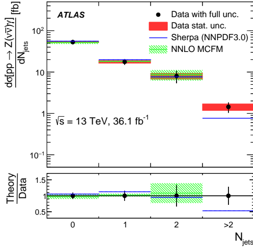
Figure 6: The measured (points with error bars) and predicted cross sections as a function of N_{\text{jets}} for the pp \rightarrow Z(v\bar{v})\gamma process in the extended fiducial region. The error bars on the data points show the sum in quadrature of the statistical and systematic uncertainties. The MCFM NNLO predictions are shown with shaded bands that indicate the theoretical uncertainties described in Section 5.4. For the SHERPA predictions, systematic uncertainty is not considered, and the statistical uncertainties arising from the size of the MC samples are too small to be visible. The lower plots show the ratios of the SM expectation to the measured values (shaded bands), with the error bars on the points showing the relative uncertainties in the experimental measurements.
