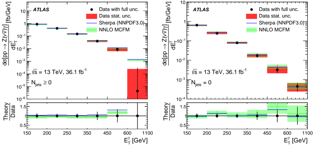
Figure 4: The measured (points with error bars) and predicted differential cross sections as a function of E_T^\gamma for the pp \rightarrow Z(\nu\bar{\nu})\gamma process in the inclusive N_{\text{jets}} \geq 0 (left) and exclusive N_{\text{jets}} = 0 (right) extended fiducial regions. The error bars on the data points show the sum in quadrature of the statistical and systematic uncertainties. The MCFM NNLO predictions are shown with shaded bands that indicate the theoretical uncertainties described in Section 5.4. For the SHERPA predictions, systematic uncertainty is not considered, and the statistical uncertainties arising from the size of the MC samples are too small to be visible. The lower plots show the ratios of the SM expectation to the measured values (shaded bands), with the error bars on the points showing the relative uncertainties in the experimental measurements. The bin size varies from 50 GeV to 500 GeV.
