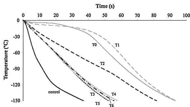
Fig. 6 Temperature evolution, during cooling by immersion in LN, of cryovials with 10 alginate beads containing mint shoot tip and treated after the encapsulation–dehydration protocol. Beads were desiccated under the air flow of a laminar flow bench for different times: T0 = 0 h (no desiccation); T1 = 1 h; T2 = 2 h; T3 = 3 h; T4 = 4 h; T5 = 5 h; T6 = 6 h; and Control = cryovial without beads. Data are the mean of at least three repeats
