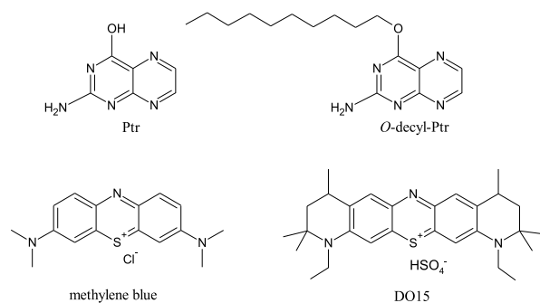
Figure 1. Chemical structure of Ptr, O-decyl-Ptr, methylene blue and DO15.
