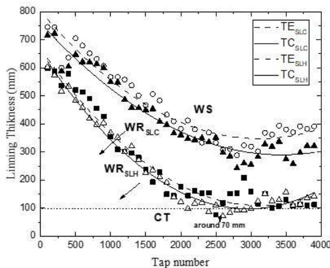
Fig- 3: Minimum lining thickness curves of the trunnions zones
