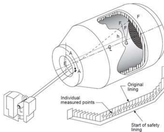
Fig-1: Scheme of the measurements practice with the laser scanner equipment [8]
