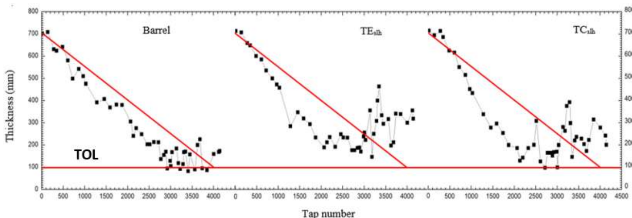
Fig-5: Screen example that shows the evolution of the Barrel, TE_{SLH} and TC_{SLH} lining thickness
