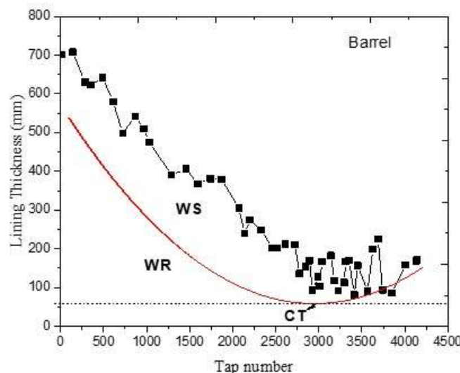
Fig-4: Barrel lining thickness evolution during a running campaign
