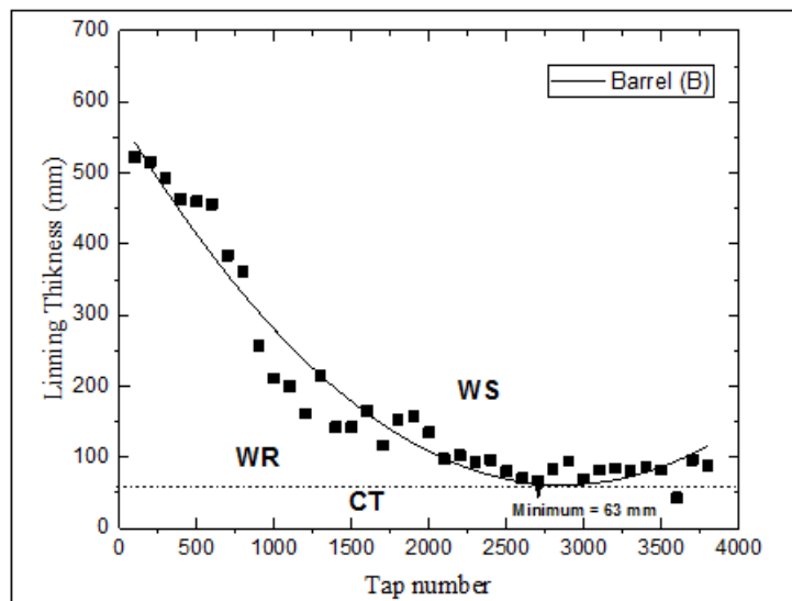
Fig-2: Minimum lining thickness curve of the barrel zone (B)
