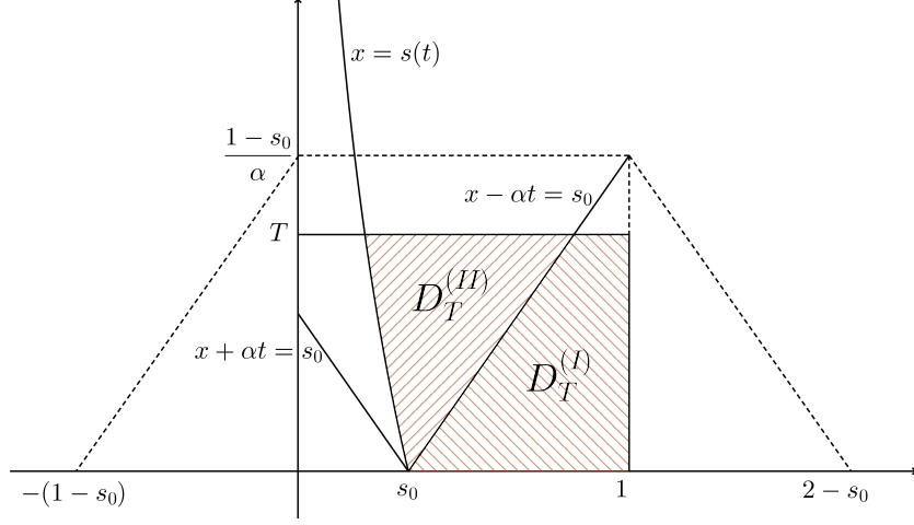
Figure 1: Schematic representation of the liquid domain D_T split into D_T^{(I)} and D_T^{(II)} .
