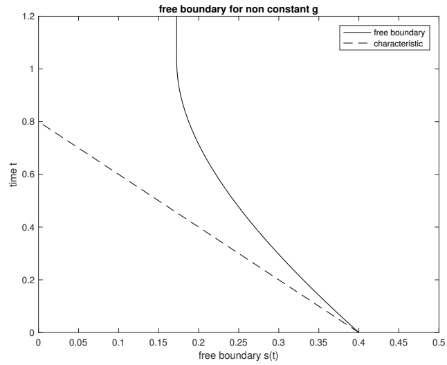
Figure 5: Free boundary x = s(t) for non constant g .
