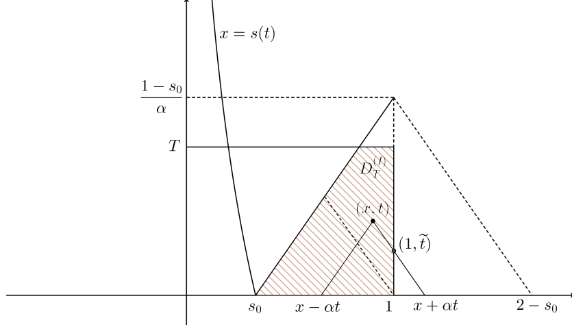
Figure 2: Characteristics lines for (x, t) \in D_T^{(I)} .
