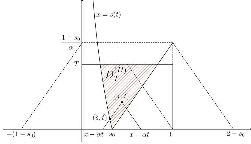
Figure 3: Characteristics lines for (x, t) \in D_T^{(II)} .
