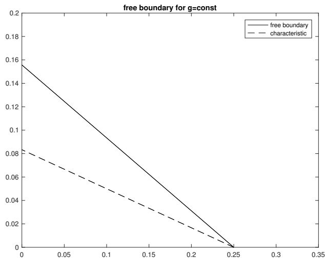
Figure 4: Free boundary x = s(t) for g = const .
