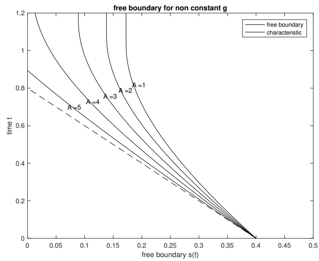
Figure 6: Free boundary x = s(t) for non constant g and A = 1, 2, 3, 4, 5 .
