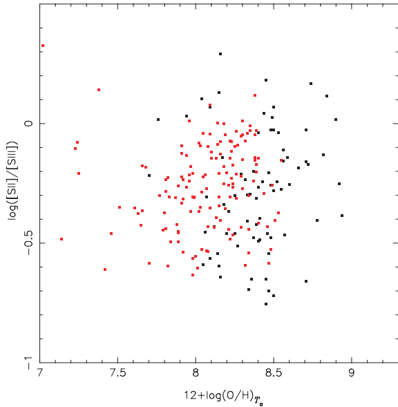
Figure 8. [\text{S II}]/[\text{S III}] observed line ratio versus oxygen abundance for the T_e -method for our sample of objects. \text{H II} galaxies and \text{H II} regions are marked with red and black squares, respectively.
