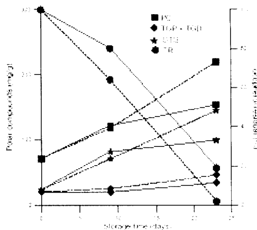
Figure 2 Evolution of polar-compound content and \alpha -tocopherol residual at 68 °C ----- control, - - - - - treated with 100 ppm of \delta -tocopherol. Abbreviations: PC = total polar compounds, TGP + TGD = total triglyceride polymers, OTG = oxidized triglyceride monomers, TR = tocopherol residual.
