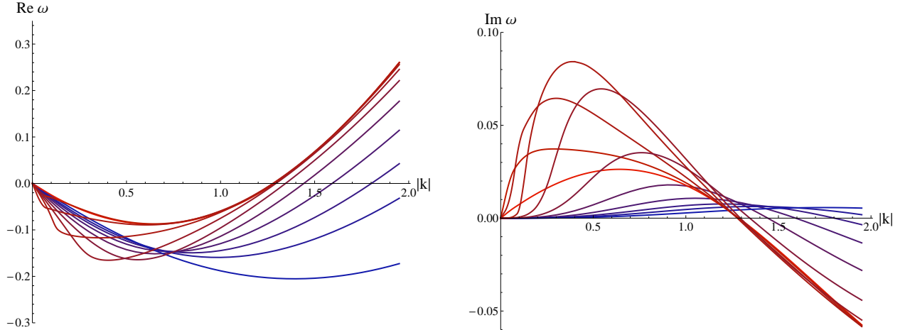
Figure 9: Real (left) and imaginary (right) parts of the dispersion relation of the lowest QNM of the (1) – (2) sector in the gauged model for fixed S_x/\mu = 0.15 and a range of temperatures from T = \tilde{T} = 0.95T_c (red) to T = 0.45T_c (blue) and momentum anti-parallel to the superfluid velocity.
