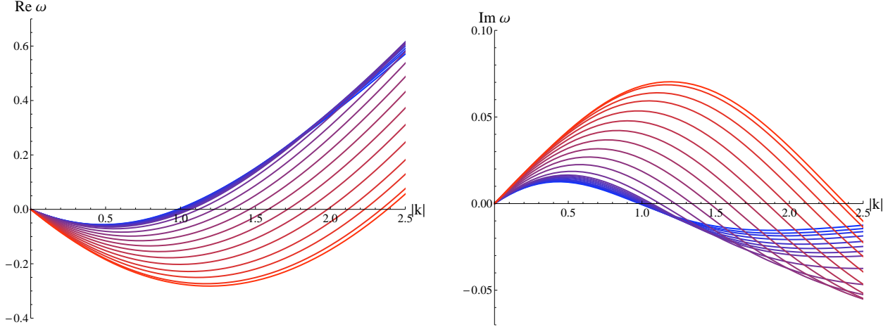
Figure 10: Real (left) and imaginary (right) parts of the dispersion relation of the lowest QNM in the (1) – (2) sector of the ungauged model for fixed S_x/\mu = 0.25 and a range of temperatures from T = \tilde{T} = 0.853T_c (red) to T = 0.306T_c (blue). Momentum is taken anti-parallel to the superfluid velocity.
