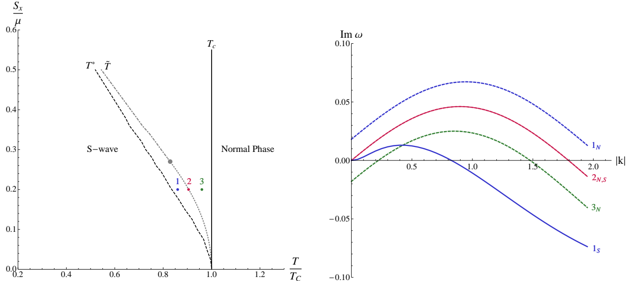
Figure 6: (Left) Phase diagram after the study of the QNMs . The grey dashed line corresponds to \tilde{T} , the apparent transition temperature found by direct analysis of the free energy. At a certain point (disk) the transition in free energy changes from 2nd order (dotted) to 1st order (dash-dotted). The black solid line corresponds to the critical temperature in absence of superfluid velocity. The black dashed line signals the physical phase transition at T^* , the temperature at which the local instability appears. Points 1, 2 and 3 indicate the values of temperature and velocity used in the plot on the right. (Right) Imaginary part of the lowest QNM for different temperatures at fixed S_x/\mu = 0.2 and \gamma = \pi . Dashed lines were obtained in the normal phase whereas solid lines were calculated in the superfluid phase.
