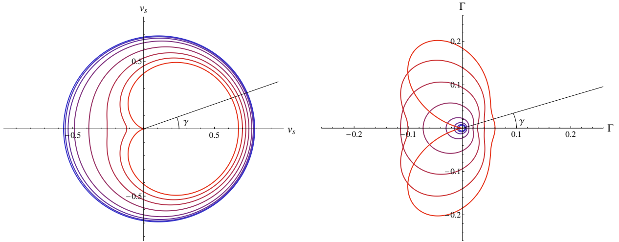
Figure 4: Sound velocity (left) and attenuation constant (right) for S_x/\mu = 0.2 as a function of the angle \gamma and for a range of temperatures from T = 0.85T_c (red) to T = 0.57T_c (blue).
