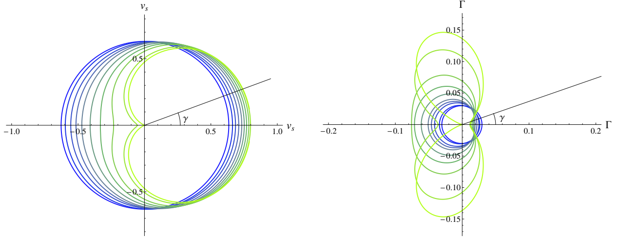
Figure 3: Sound velocity and damping for T = 0.7T_c and several superfluid velocities from S_x/\mu = 0 (blue) to S_x/\mu = 0.325 (green). The radius represents the absolute value of the sound velocity (left) and attenuation constant (right) as a function of the angle \gamma between the momentum and the superfluid velocity.
