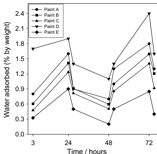
Fig. 3. Humidity adsorption-desorption cycles.
