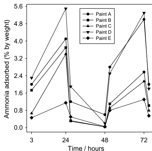
Fig. 4. Ammonia adsorption-desorption cycles.
