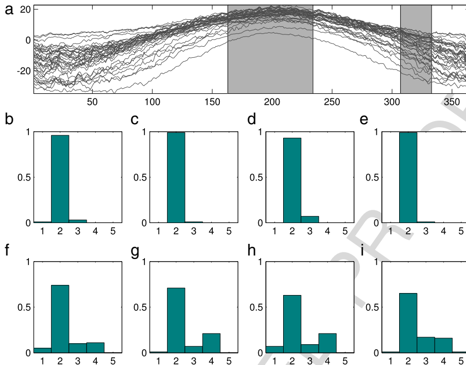
Fig. 2. (a) Temperature data set. (b)–(i) The histograms show the number of functions chosen by the algorithm for the different parameter choices. (b) r = 3, N_0 = 3, N_1 = 5 . (c) k = 3, N_0 = 3, N_1 = 10 . (d) r = 3, N_0 = 6, N_1 = 5 . (e) r = 3, N_0 = 6, N_1 = 10 . (f) r = 5, N_0 = 3, N_1 = 5 . (g) r = 5, N_0 = 3, N_1 = 10 . (h) r = 5, N_0 = 6, N_1 = 5 . (i) r = 5, N_0 = 6, N_1 = 10 .
