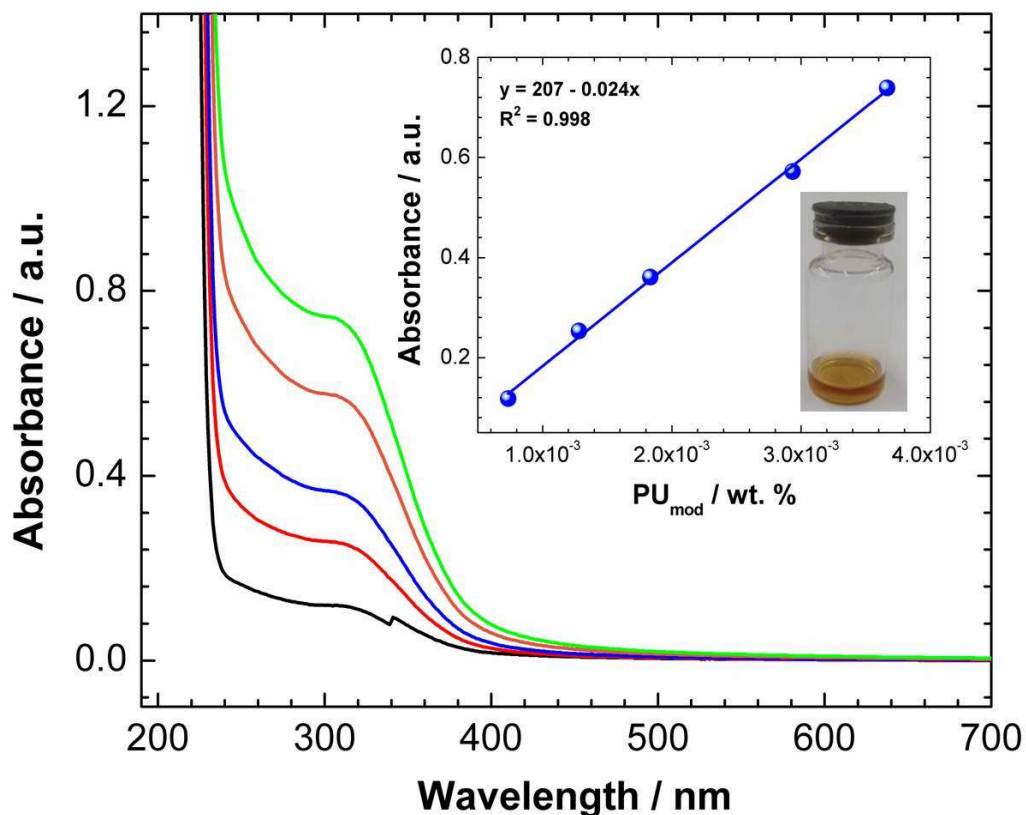
Figure 10: UV-visible spectra corresponding to PU mod dilutions. Inset: Calibration curve determined at 309 nm for PU mod . Photograph of a vial with a 3.7 \times 10^{-3} wt.% of PU mod solution.
