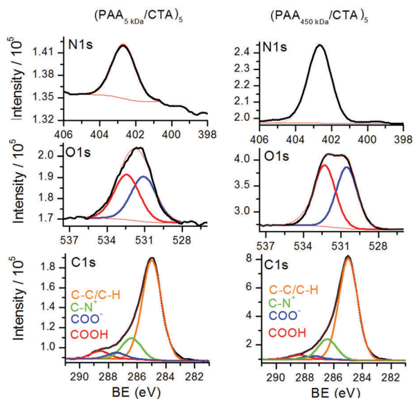
Fig. 2 X-ray photoelectron spectroscopy (XPS) O1s, N1s and C1s spectra of (PAA/CTA) 5 films prepared with low (5 kDa) and high PAA molecular weight (450 kDa). The LbL assemblies were prepared on cysteamine-modified Au substrates.
