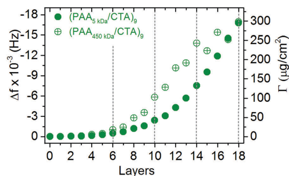
Fig. 1 Change of frequency ( \Delta f ) obtained by QCM as a function of the number of layers for (\text{PAA}_{5\text{kDa}}/\text{CTA})_n (solid circles) and (\text{PAA}_{450\text{kDa}}/\text{CTA})_n (open circles) multilayer assemblies. The frequency was measured at air atmosphere after each adsorption step. The mass surface coverage ( \Gamma ) was estimated by using the Sauerbrey's equation.
