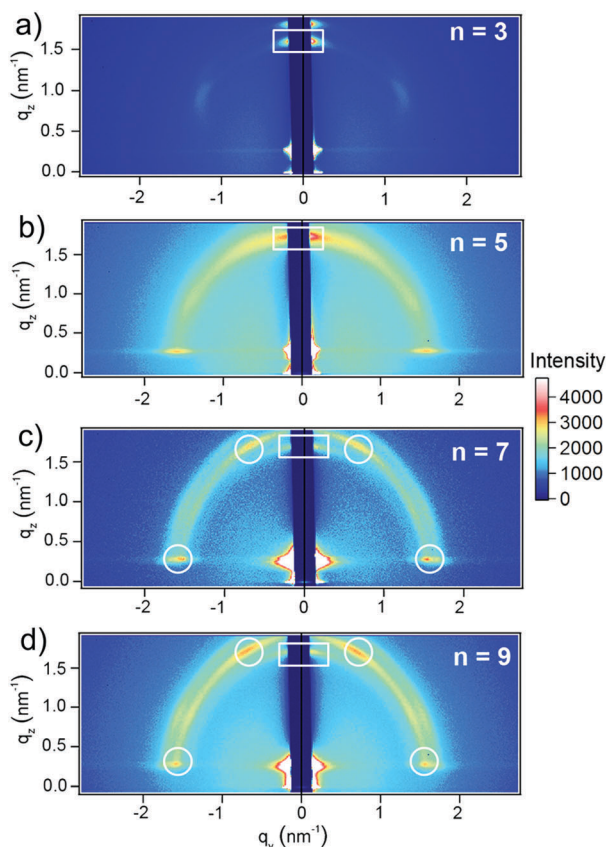
Fig. 5 GISAXS patterns obtained from (\text{PAA}_{5\text{KDa}}/\text{CTA})_n assemblies of different number of bilayers: 3 (a), 5 (b), 7 (c) and 9 (d). The films were prepared on APTES-modified Si(100) substrates and measured at an incident angle ( \alpha_i ) of 0.2^\circ . Squares show the diffraction pattern from a lamellar mesophase, while circles show the diffraction pattern from a circular hexagonal mesophase.
