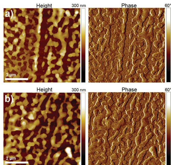
Fig. 3 AFM image corresponding to topographic (left) and phase (right) imaging of (a) (PAA 5kDa /CTA) 5 and (b) (PAA 450kDa /CTA) 5 multilayer assemblies (tapping mode; maximum z-scale: 300 nm; scan size: 6.5 μm × 6.5 μm).
