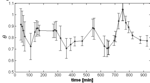
Fig. 8. Mode switching for the nominal schedule
