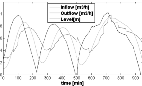
Fig. 7. Multi-modal control for the nominal schedule
