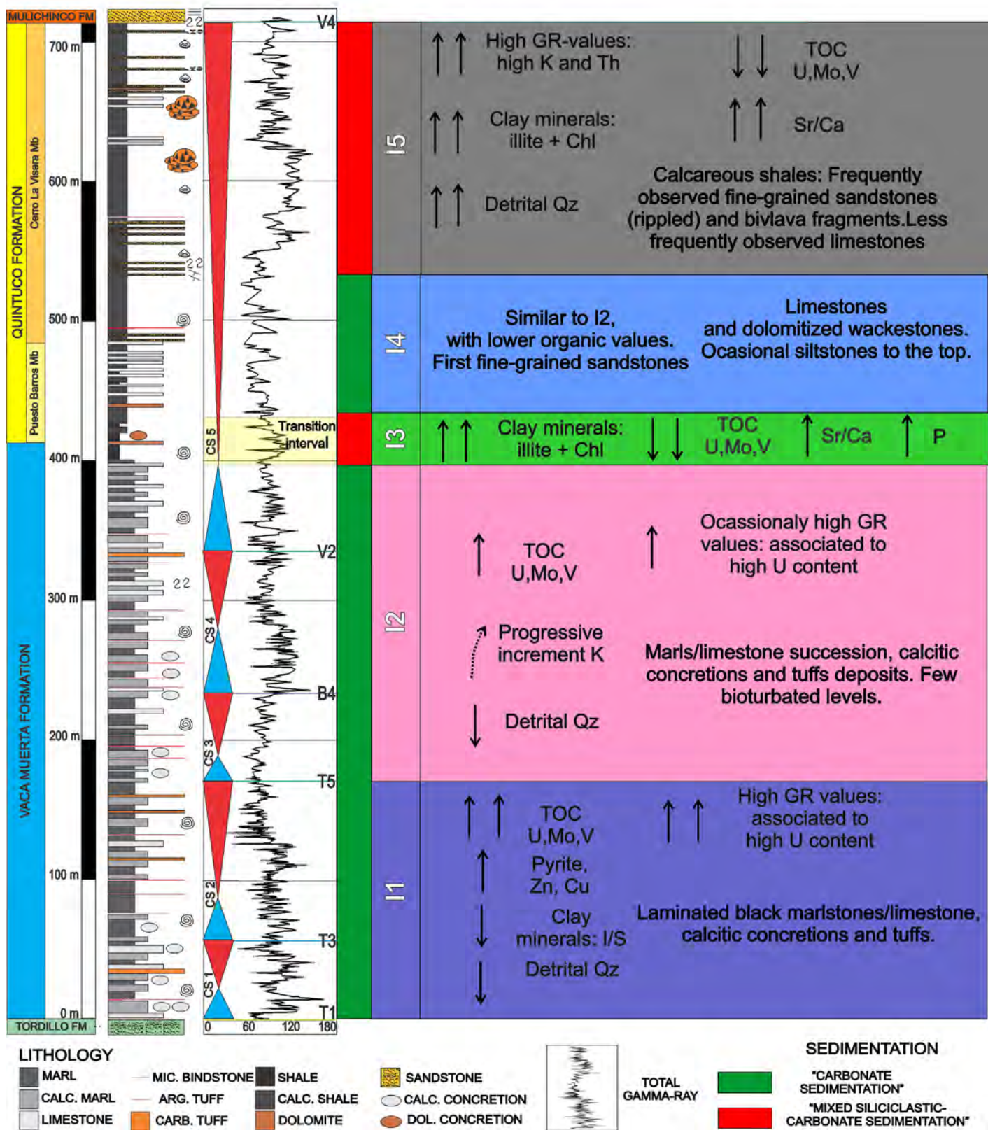
Figure 13. Schematic litholog of the Vaca Muerta-Quintuco system in Puerta Curaco area, exhibiting the main geochemical/sedimentological intervals (I1-5).
