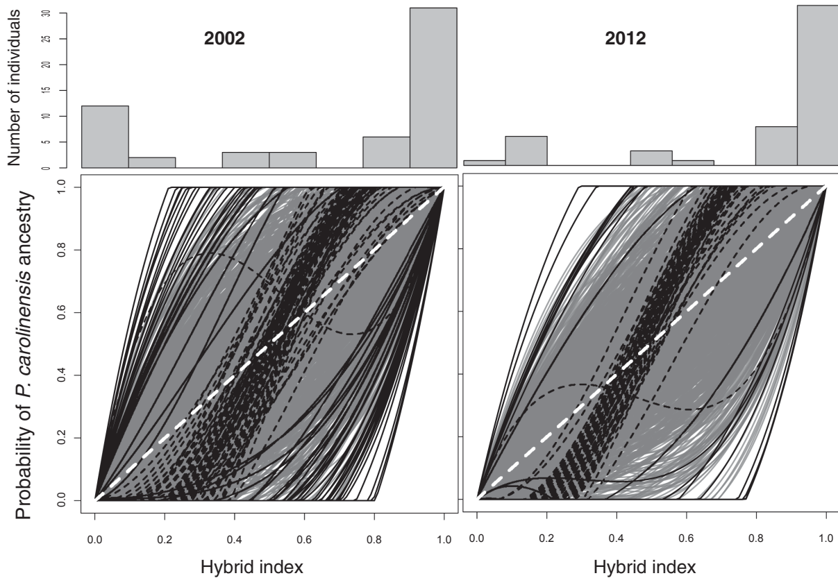
Figure 4. Estimated genomic clines for all 1425 loci in each time period. Each line represents the genomic cline for a single locus. Solid black lines indicate loci for which the 95% CI of \alpha did not include zero, dashed black lines indicate loci for which the 95% CI of \beta did not include zero, and gray lines indicate loci for which the 95% CIs of both \alpha and \beta included zero. Dashed horizontal white line gives \phi = h . Marginal histogram shows hybrid indices for the putatively admixed individuals in each time period (hybrid index of pure P. atricapillus = 0.0 and pure P. carolinensis = 1.0).
