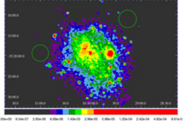
Figure 8. Highlighted with green circles two different selected background regions in the most external region of the FOV are shown. We tested the consistency of the results shown in the paper using both background regions.
