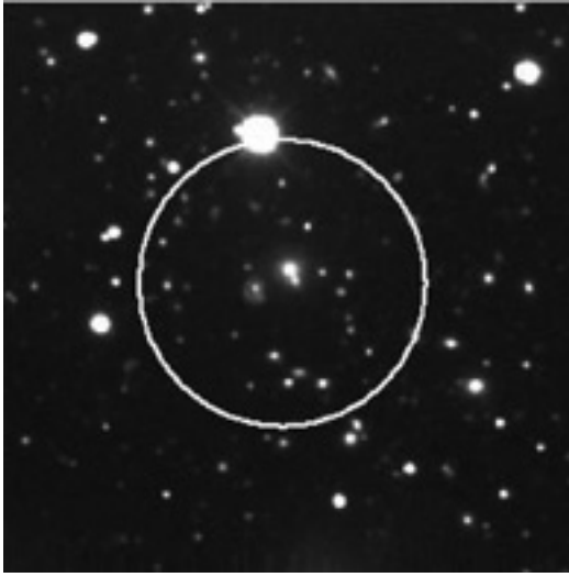
Figure 3. Combined image in C and R filters of the region around the SP of diffuse emission of the Antlia Cluster ICM. The image size is 2 arcmin \times 2 arcmin. The white circle indicates the extension of the aforementioned X-ray emission. A non-point-like optical source lies in the middle of the emission.
