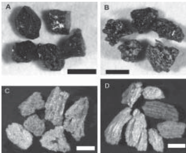
Figure 3. Examples of four major types of glassy ash particles from the August 12-15, 1991 Hudson eruption. a) blocky shards. b) low vesicular. c) highly vesicular, and d) pipe vesicular. Black and white bars are 100 microns in length.
