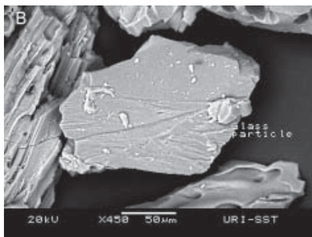
Figure 11. SEM photographs of glassy tephra particles from the August 12-15, 1991 Hudson eruption showing a) a smooth surface on a blocky particle and b) a stepped surface on a blocky particle. Scale bars are 50 microns in length.
