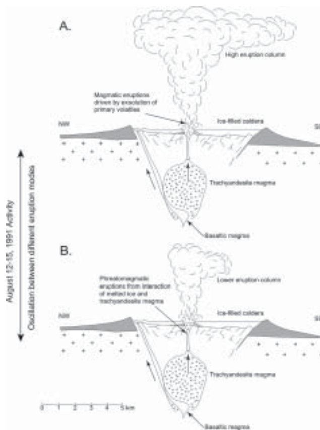
Figure 13. Suggested eruption modes during the August 12-15, 1991 climactic eruption of Hudson volcano. a). Explosive eruption of trachyandesite magma driven principally by exsolution of dissolved volatile generates high eruption column and vesicular glassy tephra. b) Interaction of meltwater from the ice-filled caldera and trachyandesite magma results in phreatomagmatic explosions that generate relatively low eruption columns and poorly-vesicular glassy tephra. Some of the interactions are likely to have occurred at depth within the conduit where the local pressure was sufficiently high to inhibit vesiculation from primary dissolved volatiles. Observed variations in eruption column height and nature of glassy particles generated during the August 12-15 period suggest oscillation between these two types of eruption mechanisms.
