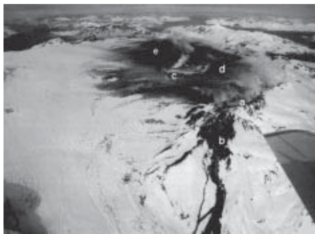
Figure 2. Aerial photograph of the Hudson caldera taken from the northwest on August 23, 1991. Basaltic dike from the August 8-10 eruption with intense fumarole activity (a) and lava flows to the northwest (b) Crater from the August 12- 15 eruption (c) bordered by a concentric pattern of ice crags (d). Dark material on the snow surface is tephra from minor explosive eruptions after August 20 (e). Photo courtesy of N.L. Banks.
