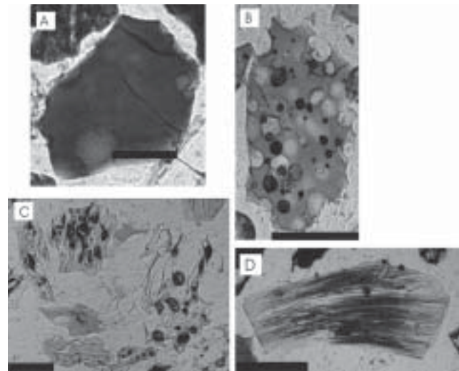
Figure 4. Transmitted light images of glass particles from the August 12-15, 1991 Hudson eruption. Note the strong contrast between different types. a) Blocky shards, dark colored and equant in shape and outlines resulting from straight to slightly irregular or concoidal fracture planes. b) Vesicular particles with low degree of vesicularity, generally equant in shape and with irregular outlines, and rounded or elongate vesicles filled by clearer fine-grained material. c) Highly vesicular particles, mostly equant in shape, with very irregular outlines and foamy texture. The outer shape of the particles is mainly the result of bubble-controlled fracturing. d) Pipe-vesicular particles are mainly whitish to light grey, show silky texture and prolated-prismatic form, sometimes twisted or bent along the «a» axis. Scale bars 100 microns long.
