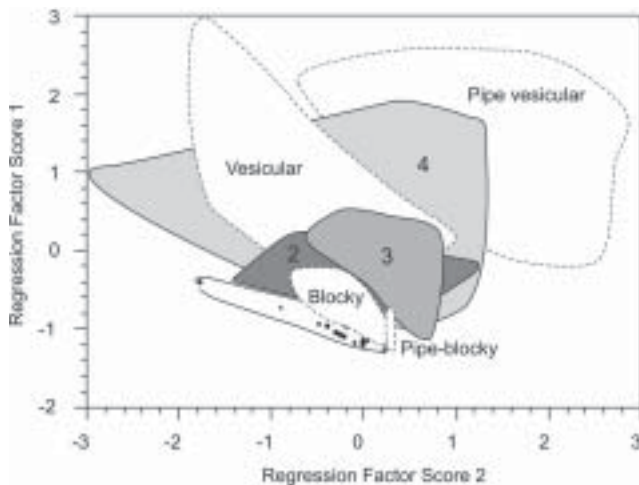
Figure 9. Comparison of Hudson tephra particles with particles from eruptions of known fragmentation mechanism based on factor analysis of fractal spectrum data. 1. Pacific seamount, 2. Surtsey (1963), 3. Katla (1918), 4. Tambora (1815).
