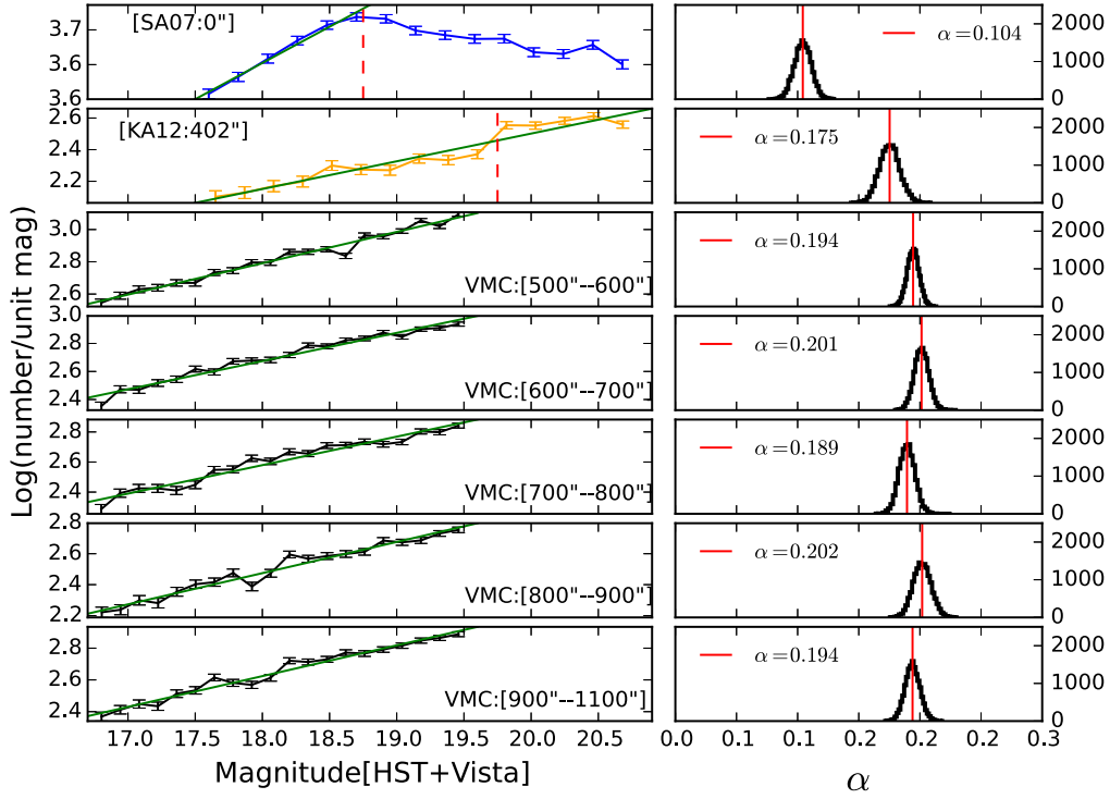
Figure 5. 47 Tuc MS LFs. LFs based on (top) the SA07 catalog for stars in the cluster center and (second panel) the KA12 catalog, containing stars located 6'7 west of the cluster center. The bottom five panels are local LFs for radial annuli covered by our VMC observations. The full annulus, r \in [500, 1100]'' , is divided into five radial subsets, i.e., r \in [500, 600]'' , r \in [600, 700]'' , r \in [700, 800]'' , r \in [800, 900]'' , and r \in [900, 1100]'' . The numbers of MS stars per unit magnitude vs. apparent magnitude F606W are plotted; the error bars were estimated based on Poissonian counting statistics. The green line is the power-law fit to the LF, and the two arrows in top two panels are an indication of a possible LF break magnitude. The Gaussian distributions on the right are the results of our Monte Carlo simulations to determine the best-fitting power-law index \alpha .
