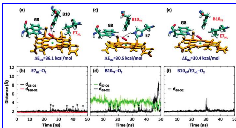
Figure 5. Schematic illustration of the distal site of representative conformations of the E7 HL , B10 YF , and B10 YF /E7 HL mutants of Ctb (panels a, c, and e). Time evolution of d_{\text{B10-O}_2} , d_{\text{G8-O}_2} , and/or d_{\text{E7-O}_2} during the 50 ns MD simulations of the O 2 -adduct of the E7 HL , B10 YF , and B10 YF /E7 HL mutants of Ctb (panels b, d, and f, respectively). The parameters d_{\text{B10-O}_2} , d_{\text{G8-O}_2} , and d_{\text{E7-O}_2} are defined as the distances between the terminal oxygen of the O 2 ligand and the hydroxyl proton of the TyrB10, the N \epsilon proton of the TrpG8, and the N \epsilon proton of the HisE7. These are depicted with red, black, and green lines, respectively. The O 2 -binding energy ( \Delta E_{\text{O}_2} ) associated with each mutant in (a, c, and e) resulting from QM-MM calculations is listed as a reference. The transient H-bonds labeled in black dotted lines in (a) and (c), associated with the structures indicated by asterisks in (b) and (d), respectively, are described in the text.
