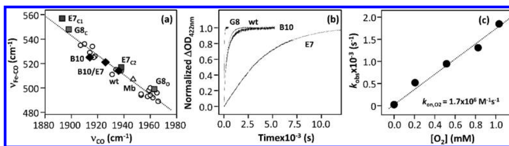
Figure 2. \nu_{\text{Fe-CO}}/\nu_{\text{C-O}} inverse correlation plot (a) and the \text{O}_2 dissociation kinetic traces (b) of the wild type and mutants of Ctb, as well as a plot of k_{\text{obs}} vs \text{O}_2 , associated with the \text{O}_2 association reaction of the \text{G8}_{\text{WF}} mutant of Ctb (c). In (a, b) E7, B10, B10/E7, and G8 stand for the \text{E7}_{\text{HL}} , \text{B10}_{\text{YF}} , \text{B10}_{\text{YF}}/\text{E7}_{\text{HL}} , and \text{G8}_{\text{WF}} mutants, respectively.
