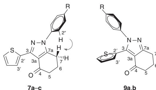
Fig. 3. Atom numbering of indazoles 7a–c and 9a,b .
