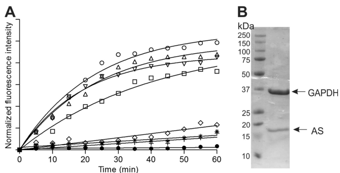
FIGURE 8. Influence of GAPDH early oligomers in the AS aggregation kinetics. A , aggregation kinetic of AS in the presence of heparin-induced GAPDH oligomers obtained after 5 min (○), 15 min (▽), 30 min (△), 60 min (□), and 24 h (*) of GAPDH-heparin interaction. Control experiments in the presence of GAPDH alone (+) and heparin (◇) are also depicted. The line represents the curve fit according to equation described under "Experimental Procedures." B , gel electrophoresis in SDS-PAGE of mixed fibrils. Protein was loaded as follows: lane 1, protein molecular weight marker; lane 2, washed fibrils. The positions of bands of GAPDH and AS are marked by arrows.
