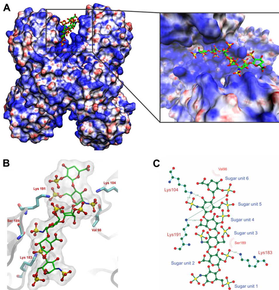
FIGURE 6. Molecular docking simulation results of GAPDH and heparin. A , front and close-up view of the protein-ligand complex. The licorice model is used to represent heparin hexasaccharide, whereas the electrostatic potential is mapped onto the solvent-accessible surface of the GAPDH; a blue color indicates a region of positive potential (+10 kT/e), red indicates a negative potential (-10 kT/e), and white indicates a neutral potential. B , binding mode of heparin to GAPDH with the protein shown in cartoon representation, with heparin and selected amino acids side chain in licorice representation. C , schematic representation of the interaction generated with Ligplot; the reducing end corresponds to the first sugar unit at the bottom of the hexasaccharide.
