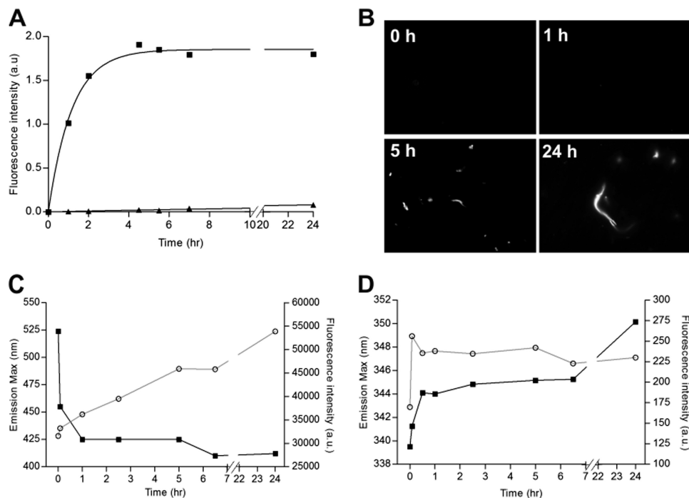
FIGURE 1. Effect of heparin on GAPDH fibrillation kinetic study by fluorescence techniques. A , GAPDH aggregation kinetics measured by thioflavin T fluorescence emission. GAPDH alone (▲) or in the presence of 75 μg/ml of heparin (■). B , thioflavin S fluorescence microscopy of GAPDH-heparin interaction at 0, 1, 5, and 24 h. Final protein concentration was 4 mg/ml and magnification 100×. C and D , changes in ANS ( C ) and Trp ( D ) fluorescence emission spectra corresponding to the fluorescence intensity (○) at the peak of the emission wavelength (■).
