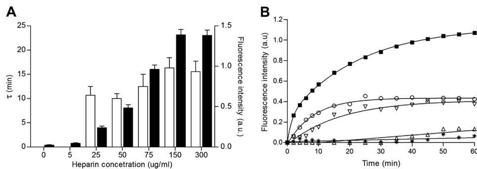
FIGURE 2. A , heparin dose dependence of GAPDH aggregation: characteristic time \tau (open bars) and final amount (closed bars) of ThT fluorescence after 1 h of incubation at 37 °C of GAPDH (0.16 mg/ml) in the presence of increasing amount of heparin. B , effect of G3P (1 mM) on heparin-induced GAPDH aggregation measured in the presence of different heparin concentrations: 75 μg/ml (*), 150 μg/ml (Δ), 300 μg/ml (▽), and 600 μg/ml (○). The GAPDH (0.16 mg/ml) aggregation kinetics induced by 75 μg/ml of heparin in the absence of G3P is also represented (■). The line represents the curve fit according to the equation described under "Experimental Procedures."
