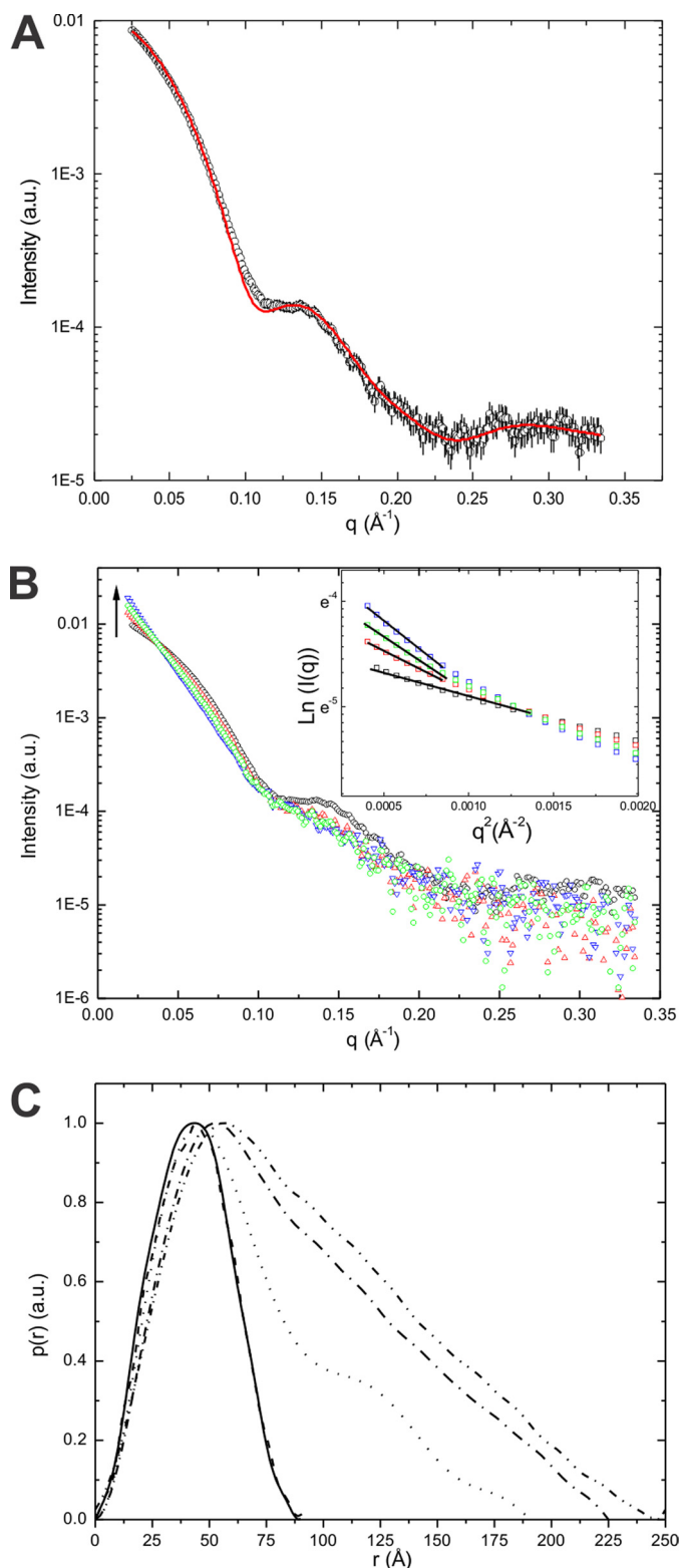
FIGURE 4. SAXS curves and data analysis of GAPDH in the presence and in the absence of heparin. A , correspondence between theoretical and experimental SAXS curves: the experimental values ( open squares ) were obtained by the scattering of 4 mg/ml GAPDH. The theoretical scattering curve ( red solid line ) calculated from the protein crystallographic structure (1J0X). B , SAXS data from 4 mg/ml GAPDH in solution in the absence ( black ) and in the presence of heparin at 2 min ( red ), 60 min ( green ), and 180 min ( blue ) of GAPDH-heparin interaction. The respective Guinier plots are displayed in the inset . C , corresponding pair distance distribution function, p(r) , calculated from the experimental scattering curve ( dashed line ) and from the
