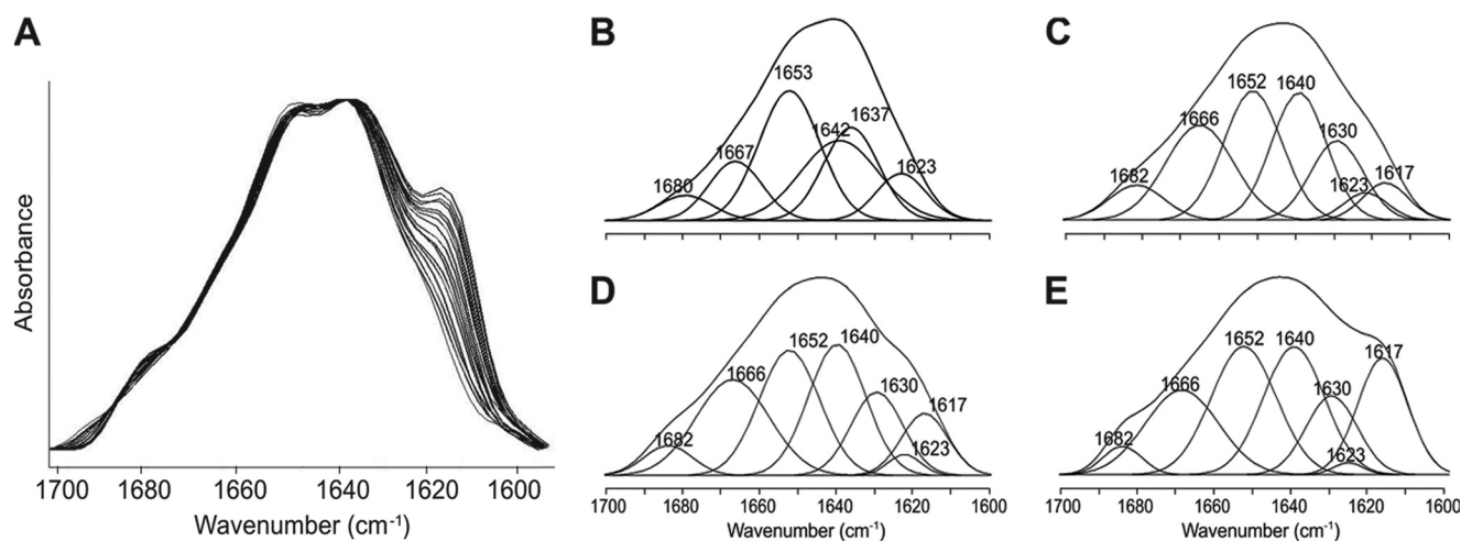
FIGURE 3. Heparin-induced GAPDH conformational changes measured by infrared spectroscopy. A , time evolution of the FTIR spectra of the deconvoluted amide I' region of GAPDH (4 mg/ml) during oligomer formation at 37 °C and pD 7. The samples were collected after 1.9 mg/ml of heparin addition in different periods of time, every 3 min until the first 60 min were reached. B–E , analysis of GAPDH amide I' band after the curve fitting procedure (see "Experimental Procedures") showing the component bands: GAPDH alone ( B ) and after 5 min ( C ), 1 h ( D ), and 24 h ( E ) of heparin addition.
