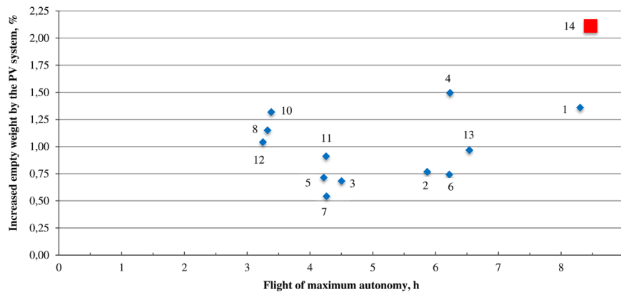
Fig. 15. Increased empty weight by install the PV system for a maximum autonomy flight per day, assuming 4 PSH, for different aircrafts.
