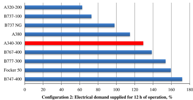
Fig. 8. Percentage of electrical demand supplied by the PV system for 12 h of aircraft continuous operation, configuration 2 cells arrangement for different aircrafts.
