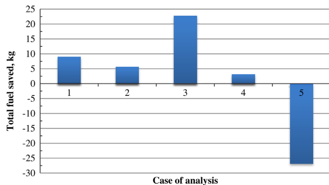
Fig. 11. Total fuel saved per type of flight according to the PV system configuration, for the cases indicated in Table 4.
