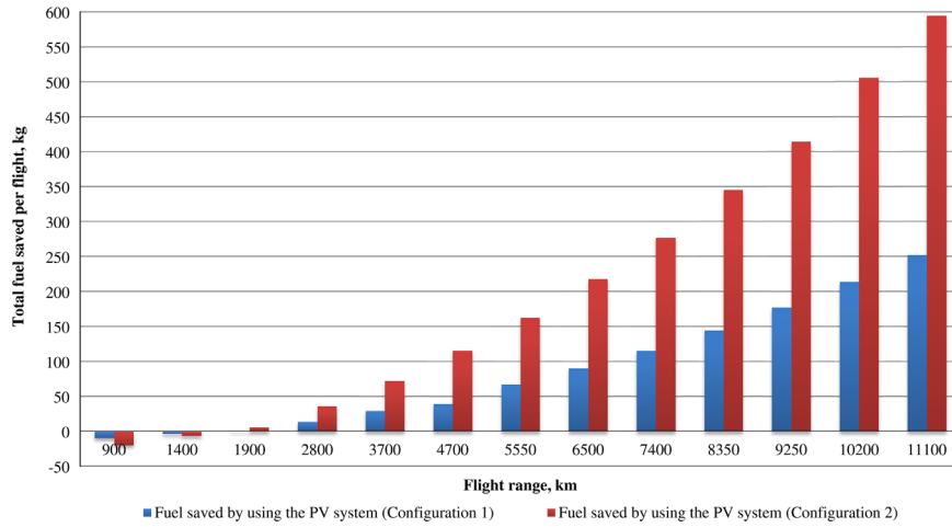
Fig. 4. Total fuel saved by type of flight and PV system configuration for the A340–300.
