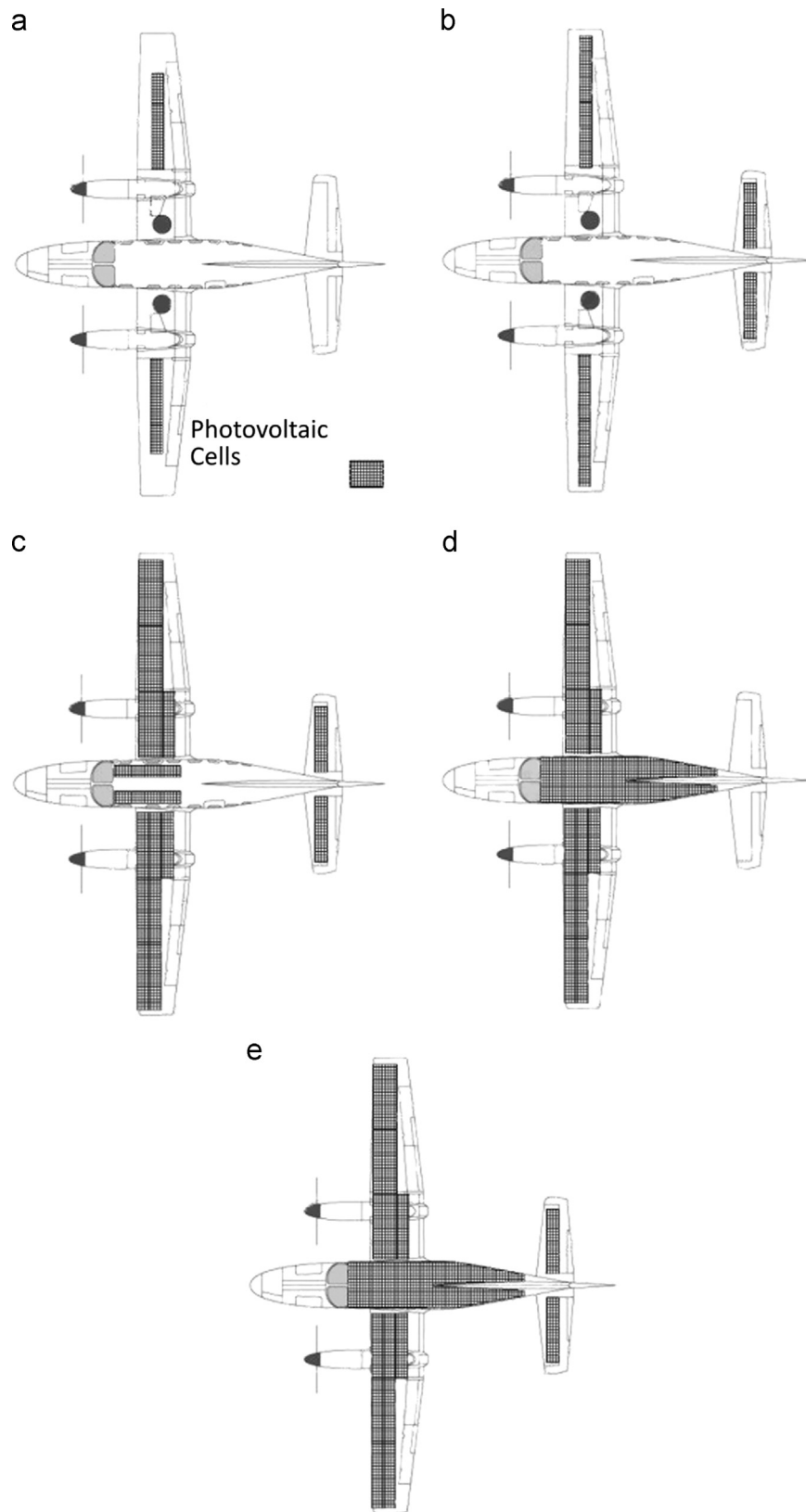
Fig. 2. Cessna Conquest 441 cell arrangement alternatives: (a) configuration 1, (b) configuration 2, (c) configuration 3, (d) configuration 4 and (e) configuration 5. The shadowed areas show the solar cells distribution on the aircraft. Source: made from http://www.the-blueprints.com/ .
