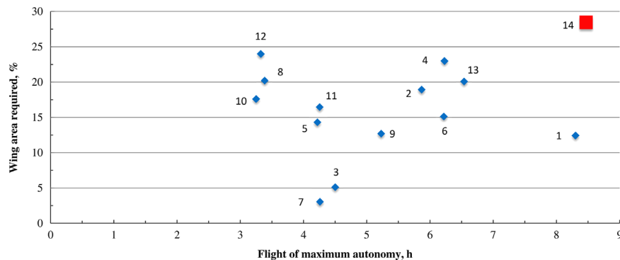
Fig. 14. Surface required by the PV system a maximum autonomy flight per day, assuming 4 PSH, for different aircrafts.
