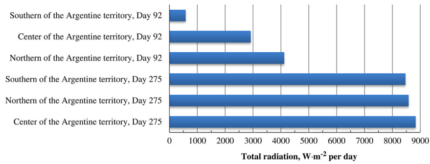
Fig. 10. Radiation on the solar cells for different scenarios in the Cessna Conquest 441, day 92 (June 21st) and day 275 (December 21st).
