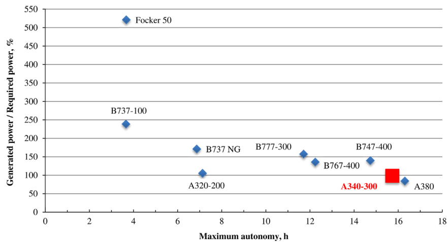
Fig. 9. Percentage of electrical demand supplied by the PV system maximum autonomy flight, configuration 2 cells arrangement for different aircrafts.
