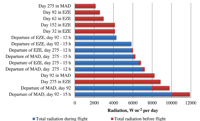
Fig. 3. Radiation on the solar cells for different scenarios in the A340–300, day 92 (June 21st) and day 275 (December 21st).
