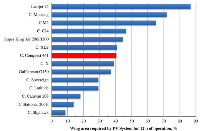
Fig. 12. Surface required by the PV system for condition of 12 h of operation per day, assuming 4 PSH, for different aircrafts.
