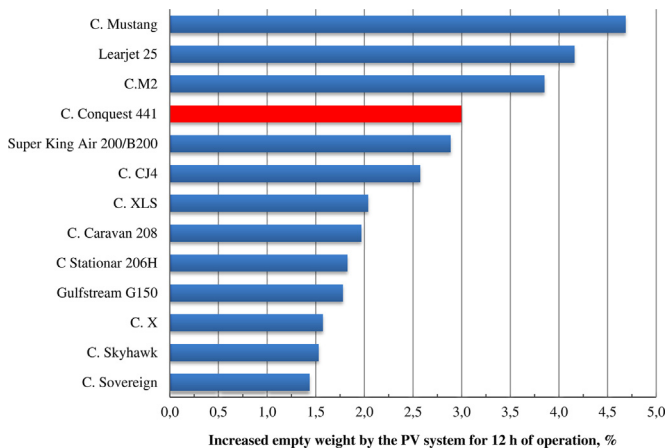
Fig. 13. Increased empty weight by installing the PV system for condition of 12 h of operation per day, assuming 4 PSH, for different aircrafts.
