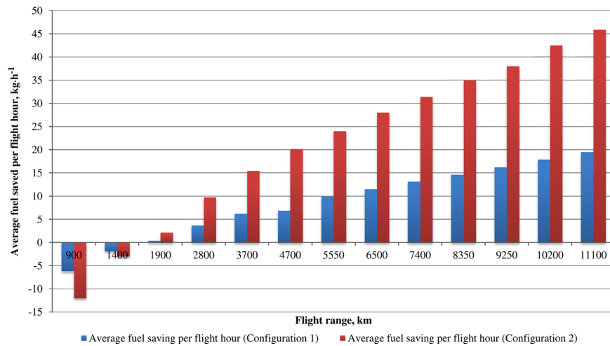
Fig. 5. Average fuel saved per flight hour by type of flight and PV system configuration for the A340–300.
