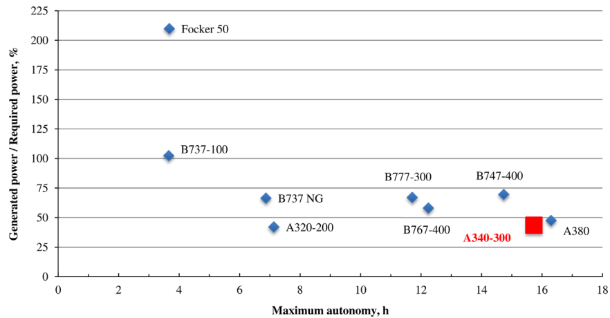
Fig. 7. Percentage of electrical demand supplied by the PV system for maximum autonomy flight, configuration 1 cells arrangement for different aircrafts.
