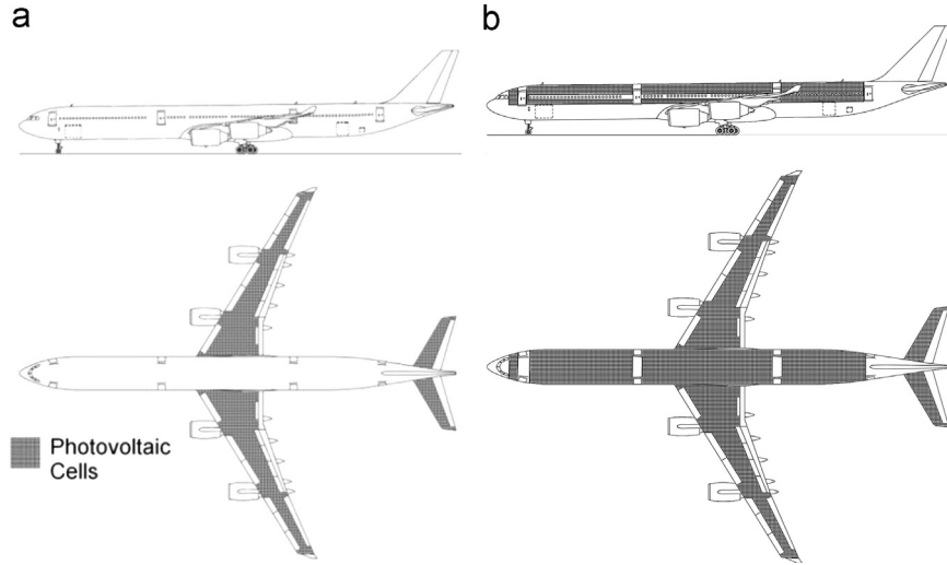
Fig. 1. A340–300 cell arrangement alternatives: (a) configuration 1, (b) configuration 2. The shadowed areas show the solar cells distribution on the aircraft. Source: made from http://www.the-blueprints.com/ .
