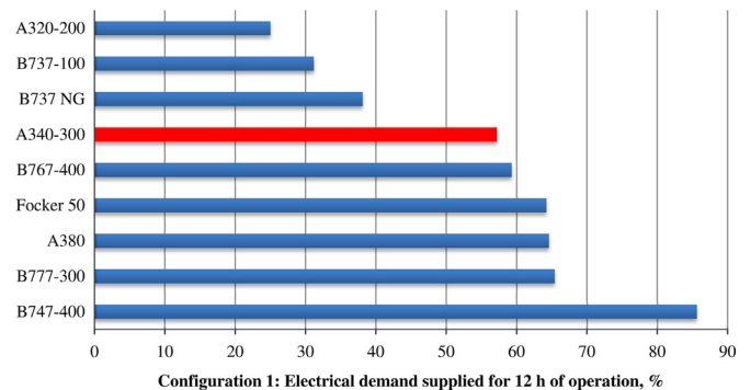
Fig. 6. Percentage of electrical demand supplied by the PV system for 12 h of aircraft continuous operation, configuration 1 cells arrangement for different aircrafts.
