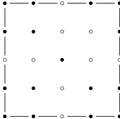
FIGURE 3. A non centrally symmetric smooth 4-selfdual configuration.
