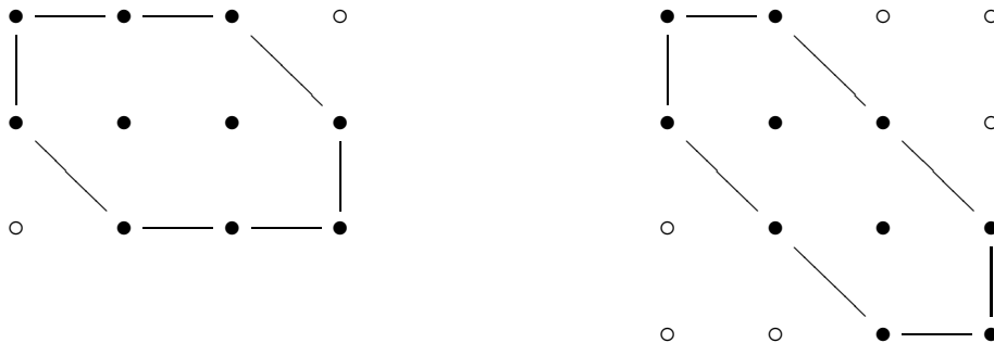
FIGURE 4. The example in § 4.3: As in [17] on the left, as in [1] on the right.
