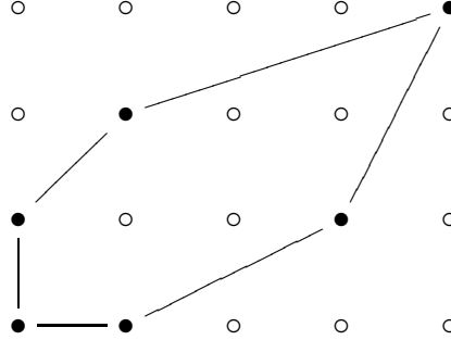
FIGURE 2. A non centrally symmetric, non smooth 2-selfdual configuration.
