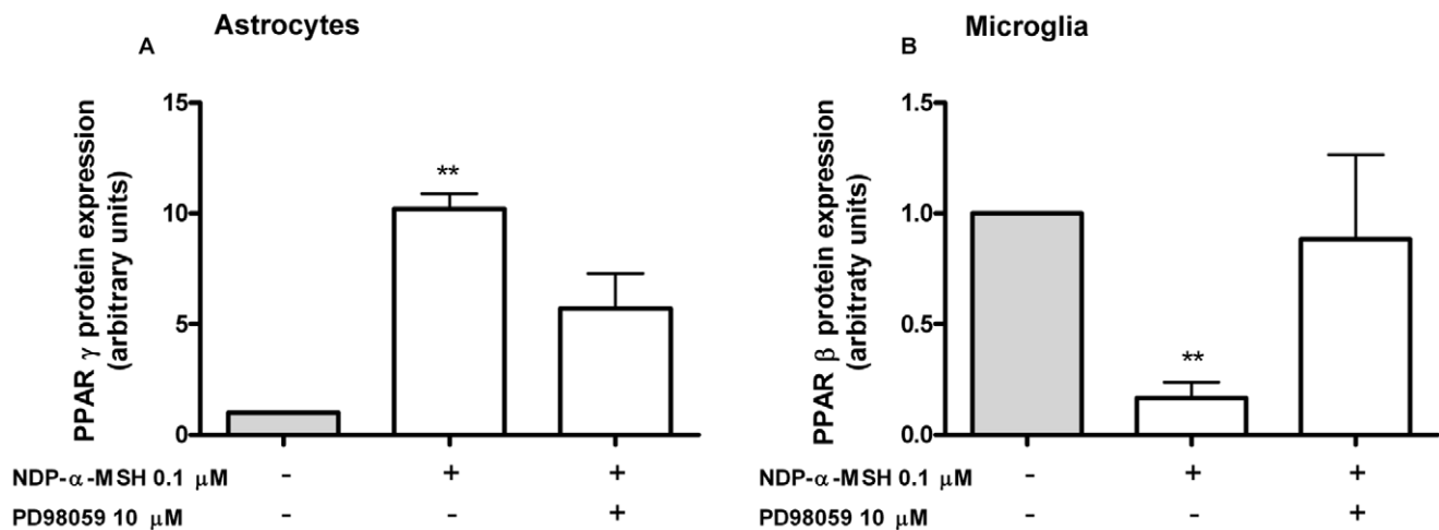
Figure 4. ERK-1/2 partially mediates the effect of NDP-α-MSH on PPAR expression. Cells were treated for 15 min with 10μM PD98059 and then 0.1 μM NDP-α-MSH was added to the culture medium. Cells were harvested after 24 h of incubation and PPAR protein levels were assessed by western blot. (A) The effect of NDP-α-MSH over PPAR-γ expression was not observed in the presence of PD98059 in astrocytes. (B) Similarly, the effect of NDP-α-MSH on PPAR-β levels was not observed in the presence of PD98059 in microglial cells. Data were analyzed by one sample t Test and are expressed as mean ± SEM. ** p < 0.01 vs. control group. doi:10.1371/journal.pone.0057313.g004
