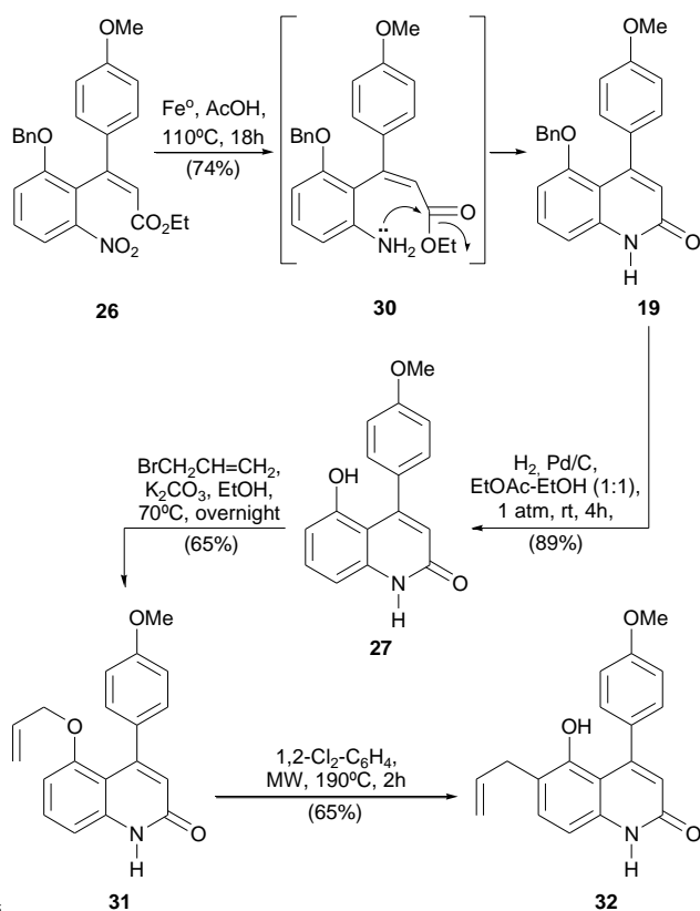
Scheme 4. Construction of the 2-quinolonic ring and synthesis of 32 .
