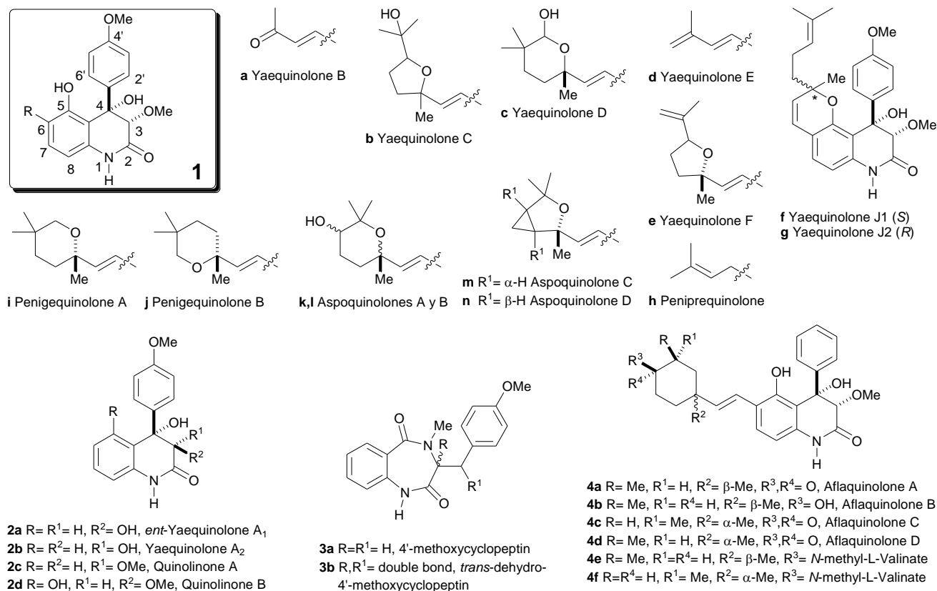
Figure 1. Chemical structures of representative naturally-occurring 6-substituted 5-hydroxy-4-aryl-1 H -quinolin-2-ones and their congeners. Except for 2a and 2d , it is assumed that the heterocycles bear a cis -3,4-dioxygenated pattern and exhibit the same 3 S ,4 S configuration.
