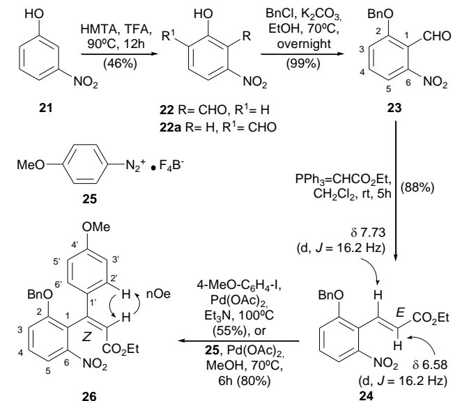
Scheme 3. Synthesis of the intermediate 26 from 3-nitrophenol ( 21 ).
