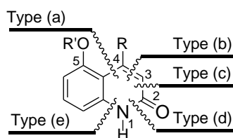
Figure 2. Most relevant general strategies for the synthesis of 4-substituted 1 H -quinolin-2-ones.
