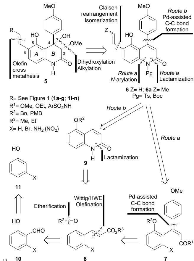
Scheme 1. General retrosynthetic analysis of the natural products 5 . Target heterocycles 6 and 6a as advanced key intermediates.
