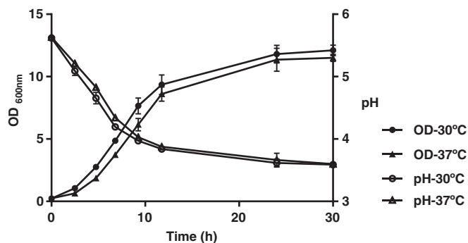
Fig. 1. Growth kinetic of L. plantarum Q823 at 30 °C and 37 °C. OD 600nm and pH trends are reported.
