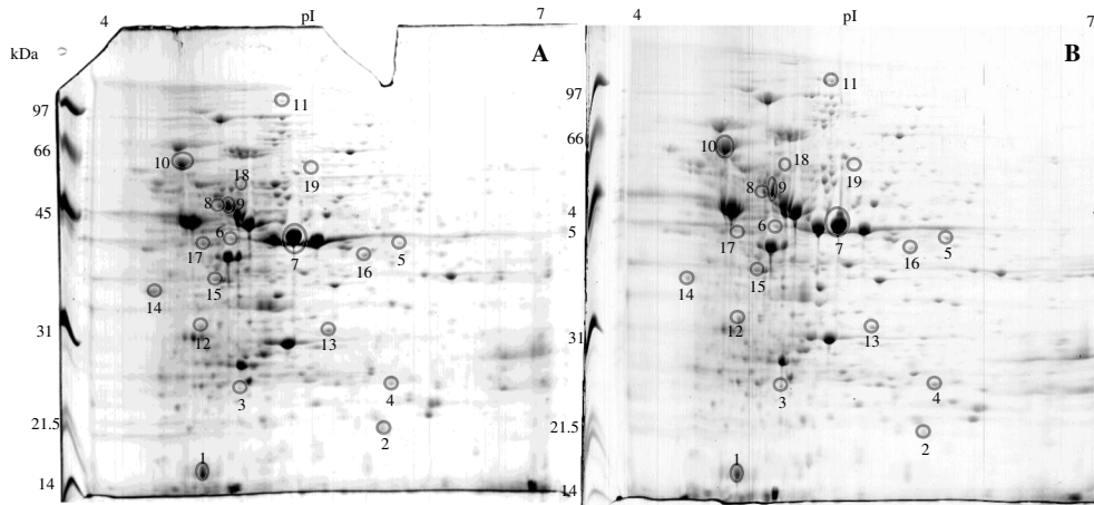
Fig. 2. Representative 2-DE gel pictures (pH range: 4–7) of in toto proteins expressed by Lactobacillus plantarum Q823 grown at 30 °C (Gel A) and 37 °C (Gel B). The differentially expressed spots are indicated.
