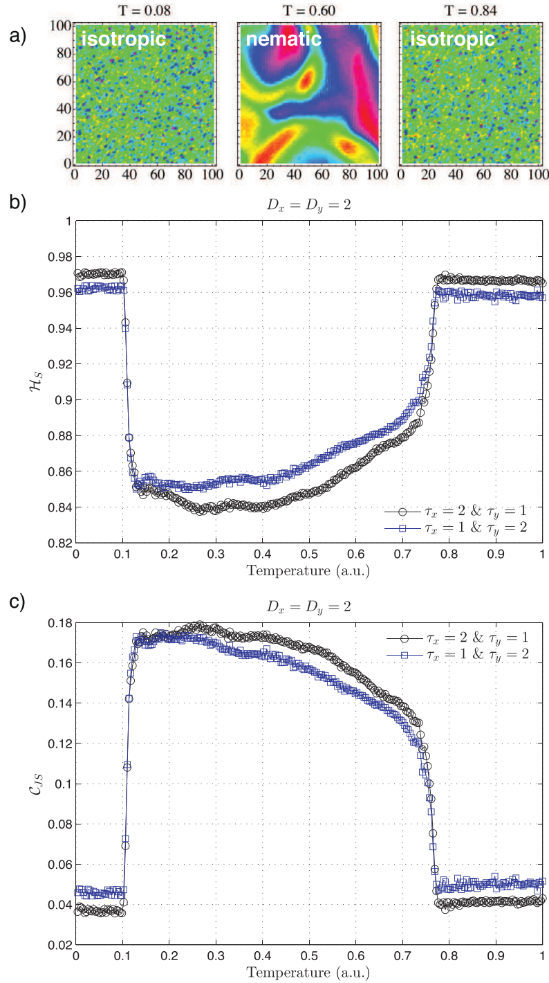
Fig. 9. (a) Examples of textures of a lyotropic liquid crystal in the (reentrant) isotropic, nematic and isotropic phases. Estimated values for (b) \mathcal{H}_S and c) \mathcal{C}_{JS} as a function of the temperature with embedding dimensions D_x = D_y = 2 and embedding delays \tau_x = 2 and \tau_y = 1 as well as \tau_x = 1 and \tau_y = 2 . (For interpretation of the references to color in this figure legend, the reader is referred to the web version of this article.)
