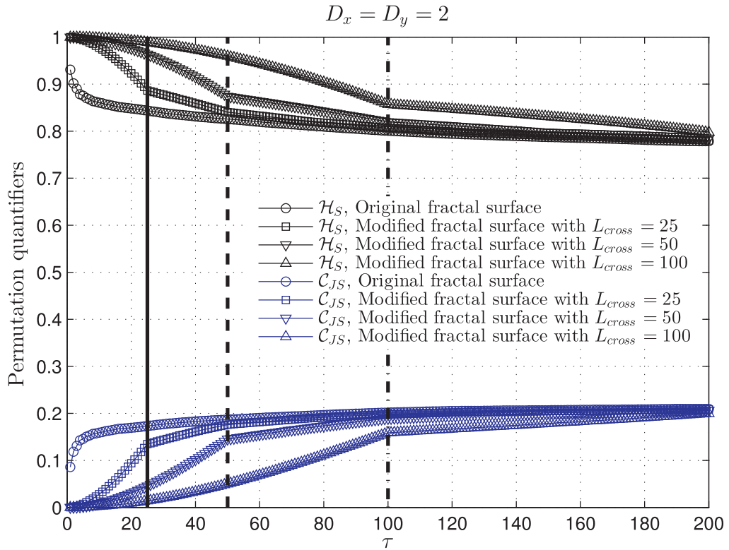
Fig. 4. Estimated \mathcal{H}_S and \mathcal{C}_{JS} as a function of the embedding delay \tau ( \tau_x = \tau_y = \tau ) with D_x = D_y = 2 for the four images displayed in Fig. 3. Vertical solid, dashed and dash-dotted black lines indicate the crossover lengths 25, 50 and 100, respectively. (For interpretation of the references to color in this figure legend, the reader is referred to the web version of this article.)
