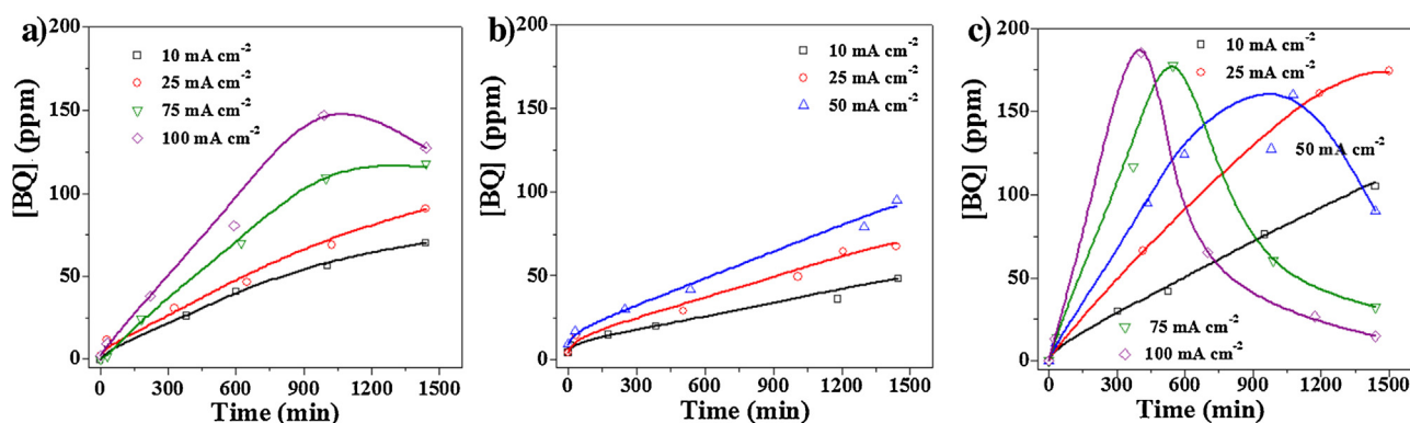
Fig. 7. Evolution of benzoquinone concentration with time during the electrochemical treatment of 1000 ppm Ph/0.5 M NaOH solution at different current densities using (a) Ti/SnO 2 -Sb(9.75)-Pt-Ru(3.25); (b) Ti/SnO 2 -Sb(3.25)-Pt-Ru(9.75); and (c) Ti/RuO 2 .
