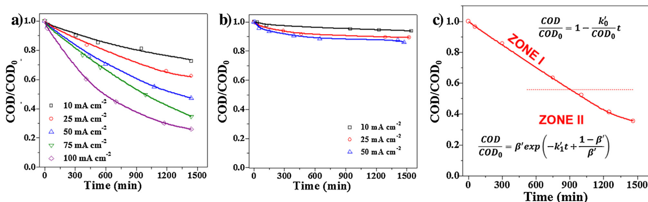
Fig. 4. Evolution of normalized COD with time for (a) Ti/RuO 2 and (b) Ti/Co 3 O 4 anodes at different current densities (electrolyte = 1000 ppm Ph/0.5 M NaOH); (c) simplified kinetic models for COD decay.
