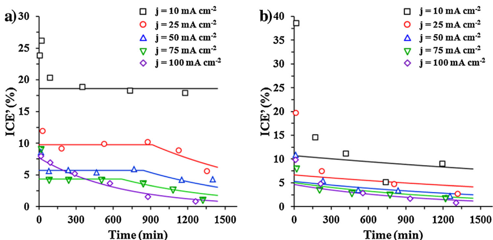
Fig. 5. Evolution of the instantaneous current efficiency (ICE') with time for (a) Ti/SnO 2 -Sb-Pt; (b) Ti/RuO 2 anodes at different current densities (electrolyte = 1000 ppm Ph/0.5 M NaOH). Open symbols represent calculated ICE' data and solid lines are the simulated model descriptions for ICE' based on fitting of experimental normalized COD data.
