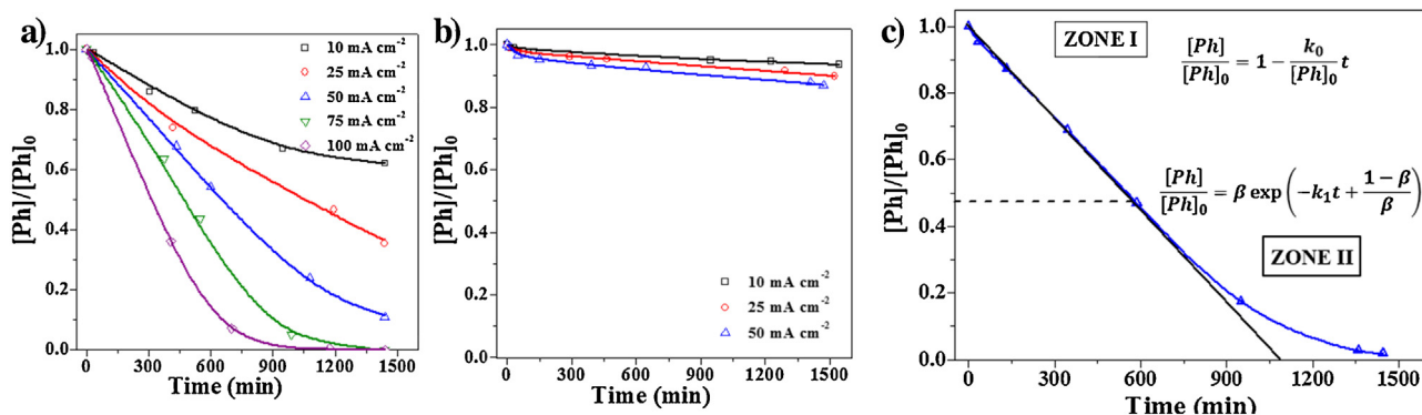
Fig. 2. Evolution of the normalized phenolate concentration with time for (a) Ti/RuO_2 and (b) Ti/Co_3O_4 anodes at different current densities (electrolyte = 1000 ppm Ph/0.5 M NaOH); (c) simplified kinetic models for phenolate decay.
