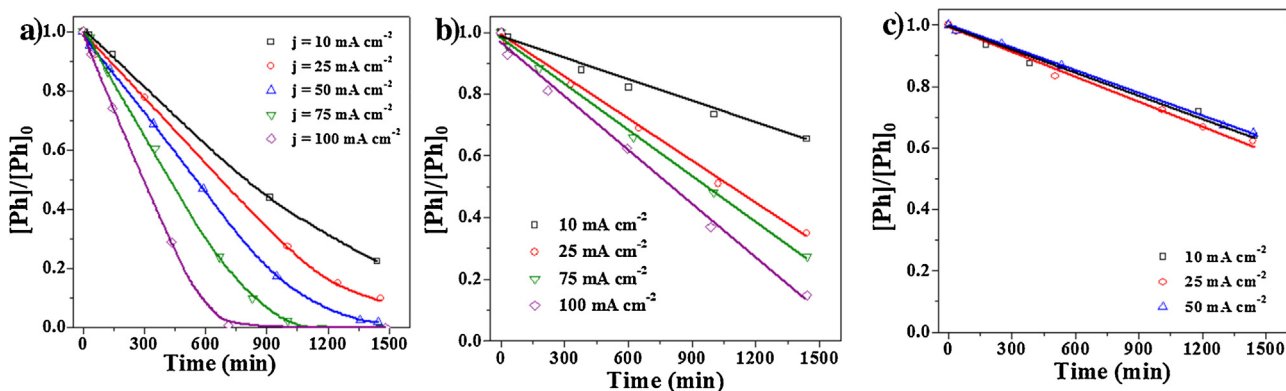
Fig. 1. Evolution of the normalized phenolate concentration with time for (a) Ti/SnO_2-Sb-Pt ; (b) Ti/SnO_2-Sb(9.75)-Pt-Ru(3.25) ; (c) Ti/SnO_2-Sb(3.25)-Pt-Ru(9.75) at different current densities (electrolyte = 1000 ppm Ph/0.5 M NaOH).
