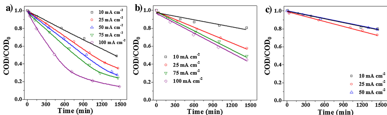
Fig. 3. Evolution of normalized COD with time for (a) Ti/SnO 2 -Sb-Pt; (b) Ti/SnO 2 -Sb(9.75)-Pt-Ru(3.25); (c) Ti/SnO 2 -Sb(3.25)-Pt-Ru(9.75) anodes at different current densities (electrolyte = 1000 ppm Ph/0.5 M NaOH).
