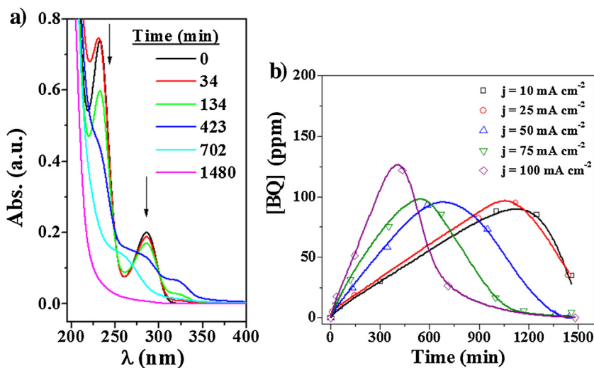
Fig. 6. Evolution of (a) UV spectrum ( 100 \text{ mA cm}^{-2} ) and (b) benzoquinone concentration (at different current densities) with time during the electrochemical treatment of 1000 ppm Ph/0.5 M NaOH solution using Ti/SnO 2 -Sb-Pt.
