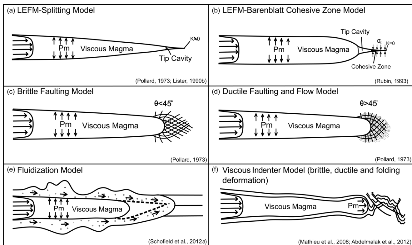
Fig. 1. Sketches of sill emplacement models. (a) Linear elastic fracture mechanics-splitting model (e.g. Pollard 1973; Lister 1990b). The overpressure ( P_m ) in the magma pushes on the sill's walls. The sill tip is expected to be sharp, and its propagation occurs by tensile opening (mode I fracturing). According to Lister (1990b), the magma viscosity is such that it does not allow the magma to flow toward the tip, leading to the formation of a tip cavity filled with fluids derived from the magma or the country rock. Tip propagation is controlled by the stress intensity factor K . (b) Elastic tensile fracture with a Barenblatt cohesive zone (Rubin 1993). This model has similarities to the former one, except that the tip propagation is controlled by the cohesion \sigma_c within the cohesive zone. (c) Brittle faulting model (Pollard 1973). In this model, the magma pushes its host rock, which fails and forms brittle faults, along which the magma subsequently propagates. (d) Ductile faulting model (Pollard 1973). Similarly to the brittle faulting model, the magma pushes its host rock, which in this case fails and forms ductile faults, along which the magma subsequently propagates. It should be noted that the angles of the shear planes differ from those expected from the brittle faulting model. (e) Fluidization model with two end-members (Schofield et al. 2010, 2012a): (i) 'thermal' fluidization, which is continuous fluidization resulting from rapid boiling of pore-fluids as magma intrudes the host rock; (2) 'triggered' fluidization, which occurs locally when heated pore-fluids are locally unconfined by opening of, for example, pre-existing fractures. (f) Viscous indenter model (Merle & Donnadieu 2000; Mathieu et al. 2008; Abdelmalak et al. 2012). In this model, the shear stresses owing to highly viscous magma flow lead to shear (brittle and ductile) failure of the host rock. In this mode, the magma appears as rigid as, or even more rigid than, the host rock.
