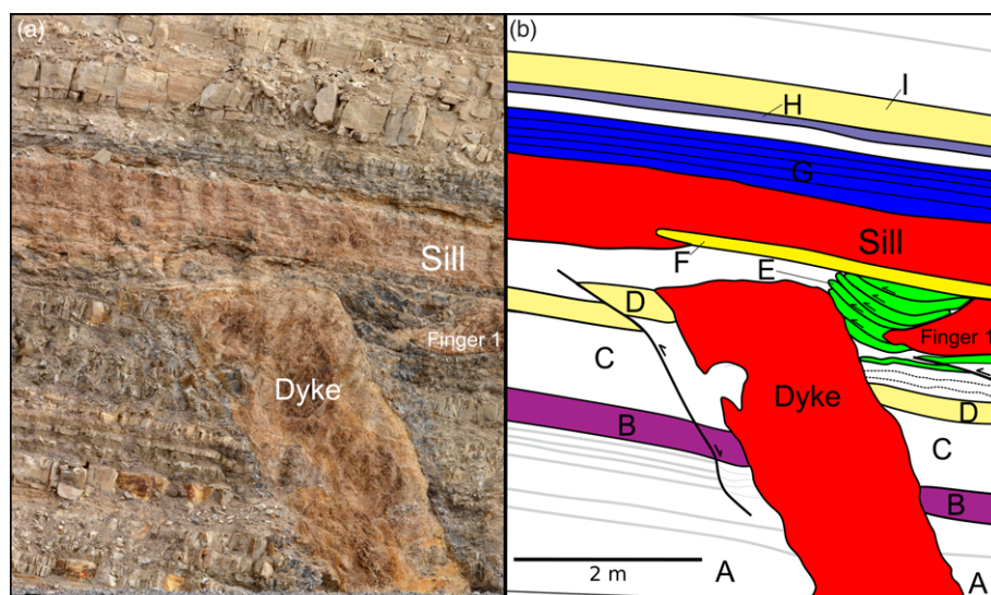
Fig. 7. (a) Detailed orthorectified photograph of the Chihuido outcrop (see location in Fig. 3), displaying the dyke and parts of finger 1 and the sill, and the surrounding structures in the host rock. (b) Detailed map of (a), displaying parts of layers B, D, E, F, G, H and I and their associated structures. The most noticeable features are (1) the multiple repetitions of layer E between the dyke and finger 1, and (2) the offset of layers B and D on the two sides of the dyke whereas layers G–I are continuous.
