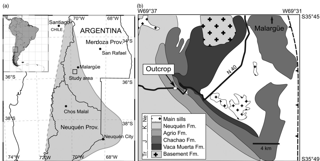
Fig. 2. (a) Regional location of the study area. (b) Simplified geological map showing location of the study area at Cuesta del Chihuido (small white rectangle).
