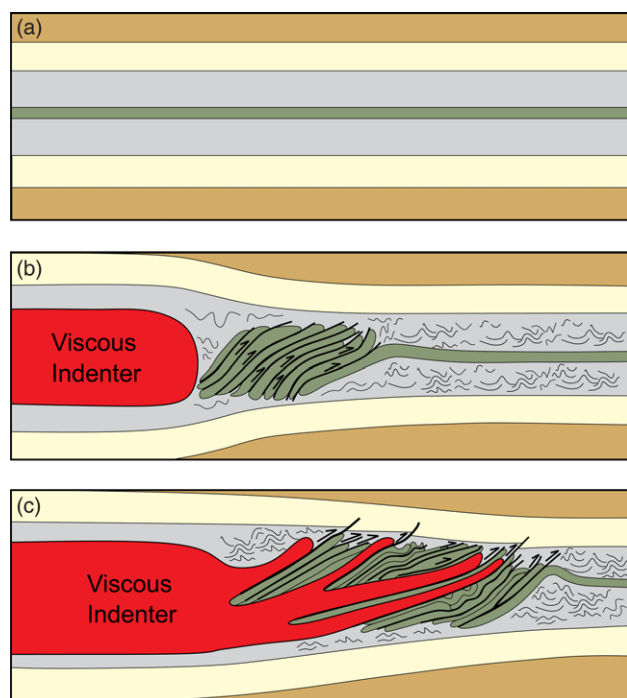
Fig. 8. Sketch showing the emplacement history of the viscous indenter model. (a) Unaltered sedimentary sequence consists of four layers of differing stiffness, thickness and composition. (b) In the initial stage of emplacement, the viscous indenter is characterized by a rounded or blunt tip. As the magma pressure pushes the tip of the sill forward, shear effects are generated, which result in shortening and folding of the country rock. (c) In this manner the sill propagates by indenting the country rock. The end result is a sill with a high radius of curvature of its tip; also, the compression exerted on the country rock generates folds, faults and repetition of layers.
