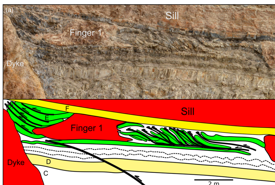
Fig. 5. (a) Detailed orthorectified photograph of the Chihuido outcrop (see location in Fig. 3), displaying finger 1 and parts of finger 2, sill and dyke, and the surrounding structures in the host rock. (b) Detailed map of (a), displaying parts of layers C, D, E and F and their associated structures. The most noticeable feature is the numerous repetitions of layer E between the intrusions.
