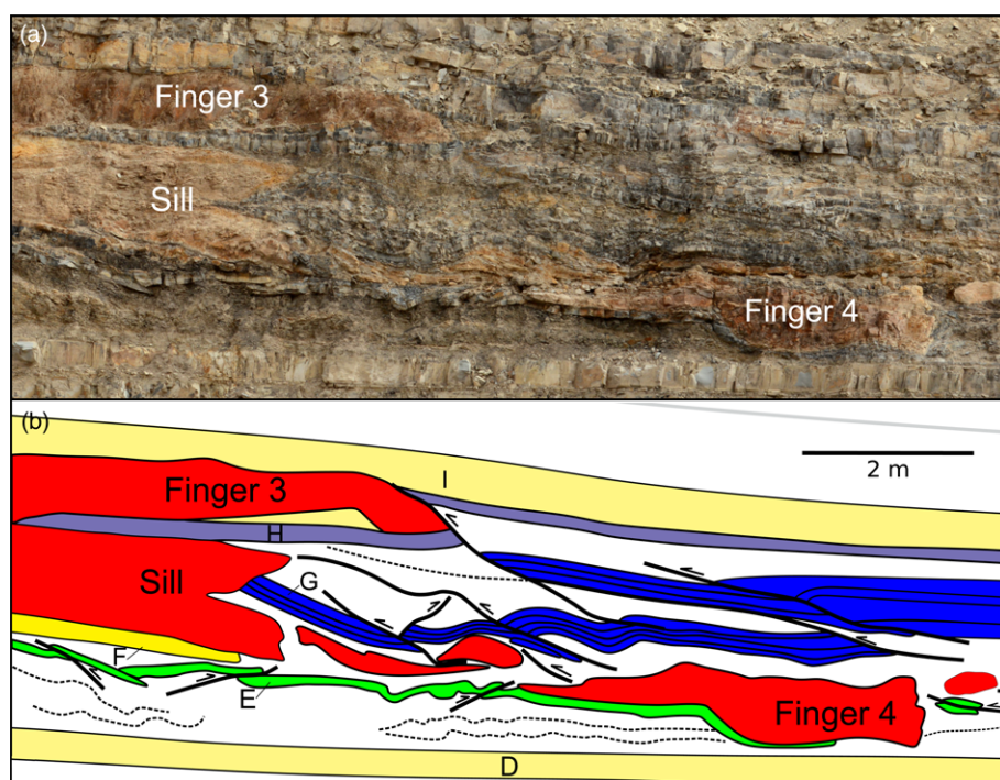
Fig. 4. (a) Detailed orthorectified photograph of the Chihuido outcrop (see location in Fig. 3), displaying fingers 3 and 4 and part of the sill, and the surrounding structures in the host rock. (b) Detailed map of (a), displaying parts of layers D, E, F, G, H and I and their associated structures. The most noticeable feature is the repetitions of layer G.
