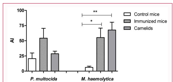
Figure 4: Avidity test. To analyze the sera avidity, ELISAs for both bacteria using 8M urea as dissociating agent were performed. The avidity index (AI) for each serum studied was calculated according to description in materials and methods. Results were expressed as mean AI \pm SEM for each group. *P<0.05; **P<0.01.
