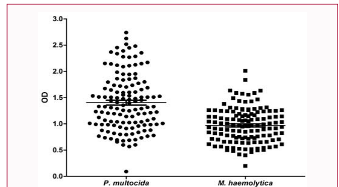
Figure 1: Antibodies against P. multocida and M. haemolytica in camelid sera. A single dilution for each serum sample was analyzed by indirect ELISA. Optical density (OD) values obtained for each bacterium are shown.
