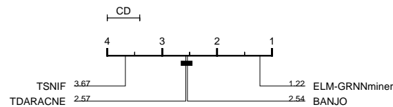
Fig. 6: Critical difference diagram for F-measure in all datasets.
