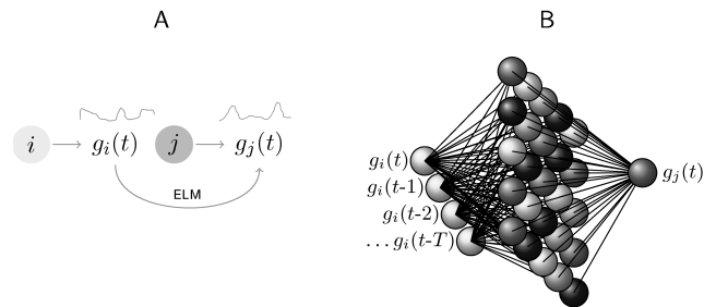
Fig. 1: Modeling a gene-to-gene regulation with ELMs. A) A possible g_i -to- g_j regulation that can be modeled with an ELM. B) ELM random projections from g_i -to- g_j time series data, by considering T time delays of g_i at the input.
