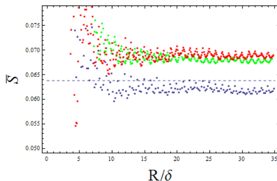
Figure 5. The averaged constant term in the entropy of circles \bar{S}(R) in a square lattice as a function of the radius in lattice units, R/\delta . The blue points are for a radius step \Delta R = 0.2 (as in figure 1). The red points are for \Delta R = (3\pi)^{-1} \sim 0.106 . The green points are for the same \Delta R but the circles are centered at the point (1/3, 1/2) in lattice units, rather than at the origin. The correct value of 2\pi c_0 is shown with the dashed line.
