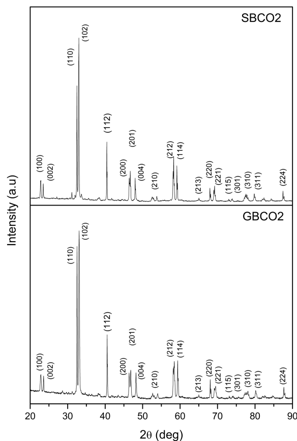
FIG. 1. X-ray diffraction patterns for the samples SBCO2 and GBCO2 treated at 1050°C. Data corresponds to single phase samples with orthorhombic crystal structure of Pmmm space group. Only in the case of SBCO2 sample, the presence of \text{BaCoO}_{2+\delta} impurity was detected (see text).
