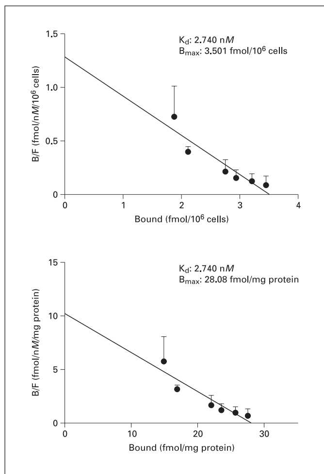
Fig. 1. Scatchard plot of [^3\text{H}] muscimol binding to TM3 cells. Results of muscimol binding to TM3 cells (one of two experiments yielding almost identical results) is shown and results are expressed per cell number and protein content.
