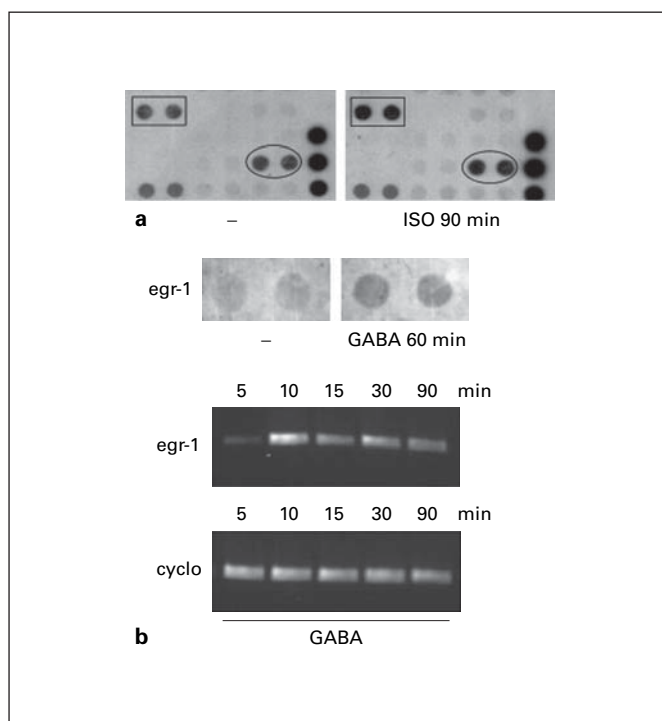
Fig. 2. Results from cDNA array studies and RT-PCR. a Example result from cDNA array studies showing that c-fos (boxed) and heat shock factor (hsf-1; circled) mRNA levels are increased 2- to 3-fold after 90 min of isoguvacine (ISO) treatment ( 10 \mu\text{M} ; duplicate blots). Compare with table 1, in which results after 120 min are summarized and imply dynamic regulation of e.g. hsf-1. b Upper panel: Result from cDNA array study showing that egr-1 mRNA levels are increased after 60 min of GABA ( 10 \mu\text{M} ) treatment (duplicate blots). Lower panel: Semiquantitative RT-PCR showing egr-1 mRNA expression levels in TM3 cells from 5 to 90 min after 10 \mu\text{M} GABA treatment (1 representative of 3 independent experiments). Cyclophilin A (cyclo) expression at the same time points as control of potential loading differences.
