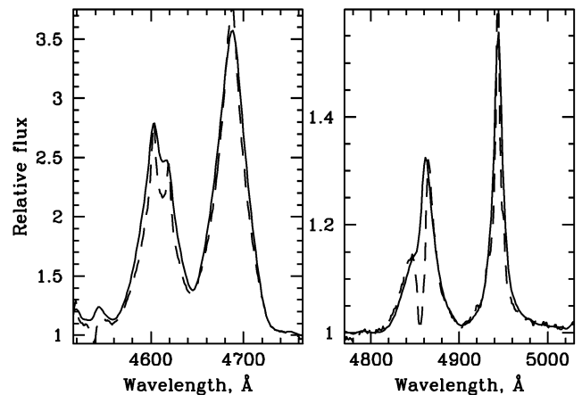
FIG. 5.—Average spectrum of WR 46 ( solid lines ) compared with the averaged WR 3 spectrum ( dashed lines ). The initially higher resolution WR 3 spectrum was convolved with a Gaussian instrumental profile corresponding to the configuration used for WR 46. In addition, the WR 3 spectrum was multiplied by a constant value (2.03) to match the intensities of the WR 46 profiles.
