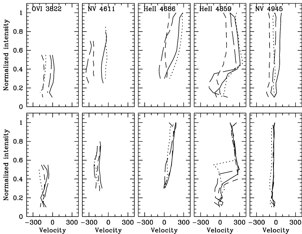
FIG. 14.—Bisectors of prominent emission lines calculated for the I_{\min}, \dots, I_{\max} line intensity ranges and in 0.05I_{\max} steps, where I_{\max} is a maximum line intensity; I_{\min} and f are chosen to avoid blending problems. The bisectors were calculated for the individual spectra ( top , night 3, moving case; bottom , night 2, nonmoving case) taken \Delta\phi \sim 0.25 apart. The solid lines denote the bisector for \phi \sim 0.0 , the dotted lines mark the bisector for \phi \sim 0.25 , the short-dashed lines mark the bisector for \phi \sim 0.5 , and the long-dashed lines denote the bisector for \phi \sim 0.75 .
