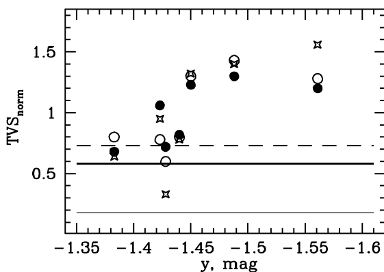
FIG. 13.—Dependence of the line-integrated, rescaled TVS on the nightly averaged continuum flux. Open circles , the O VI doublet; stars , the He II + N V complex; filled circles , the N V \lambda 4944 profile. Dashed, thick, and thin solid lines provide the 95% detectability levels for the aforementioned lines, respectively.
