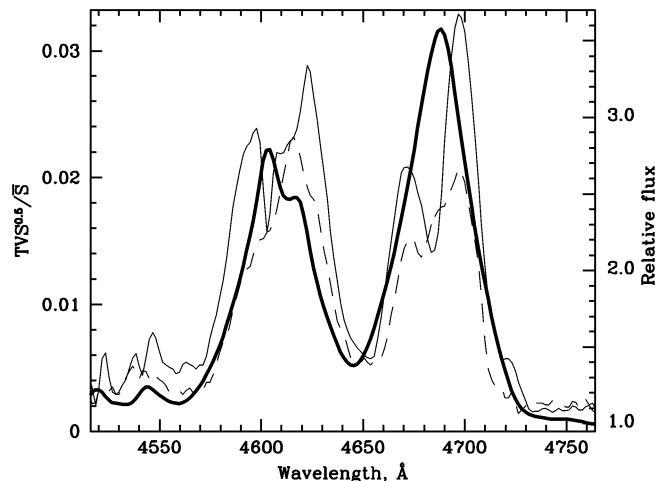
FIG. 9.—Comparison of the rescaled TVSs. Thin solid line , average of TVSs from nights 3, 4, 6, and 7, i.e., the moving case; dashed line , average nonmoving TVS for nights 1, 2, and 5; thick line , mean WR 46 spectrum.
