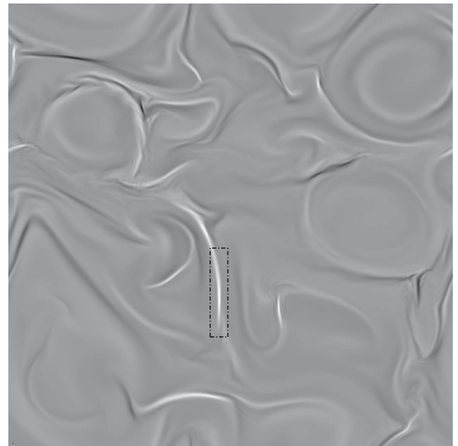
FIG. 6. Parallel component of the current density in a perpendicular plane to the external magnetic field in the case with \epsilon = 0 . Tones indicate out of plane current, with light tones = positive and dark tones = negative.
