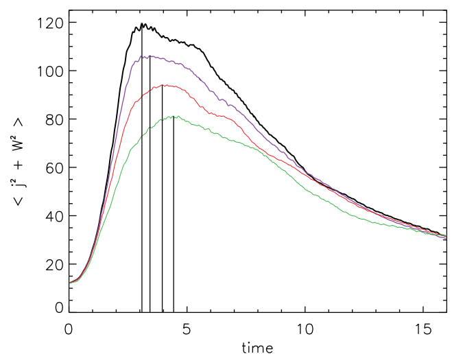
FIG. 3. \langle J^2 + \omega^2 \rangle as function of time for \epsilon = 0, 1/32, 1/16, and 1/8 . We are using the same convention of color/thickness than in Figure 1. The vertical straight lines indicate the maximum value for each curve.
