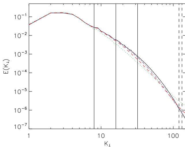
FIG. 4. Energy perpendicular spectra for \epsilon = 0 (solid line), \epsilon = 1/32 (dashed-dotted), \epsilon = 1/16 (dashed), and \epsilon = 1/8 (dotted). The vertical straight lines indicate the different values of K_{Hall} = 1/\epsilon for \epsilon = 1/32, 1/16, 1/8 . The vertical straight dashed lines show the minimum and the maximum values of the K_{diss} ( \epsilon = 1/8 and \epsilon = 0 ), through them we can see the effect of the Hall term on the dissipation scale.
