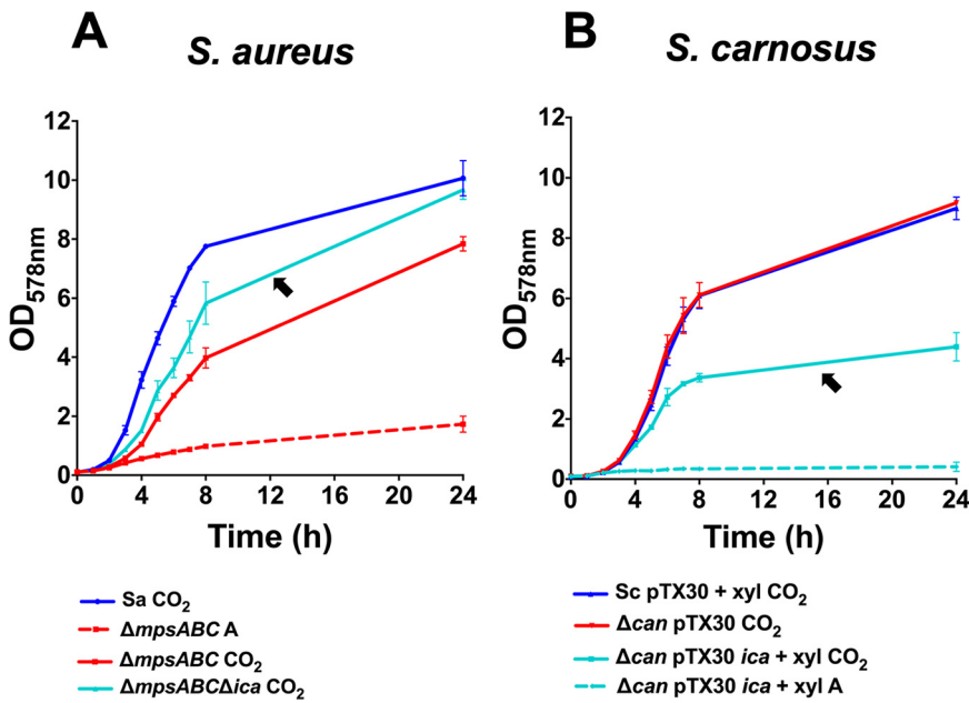
FIG 4 The influence of biofilm mediated by polysaccharide intercellular adhesin (PIA) encoded by the ica operon in the growth of staphylococcal strains. (A) The growth of the S. aureus HG001 wild type (Sa), HG001 mpsABC deletion mutant ( \Delta mpsABC ), and HG001 mpsABC and ica deletion mutant ( \Delta mpsABC ica ) under atmospheric (A, dashed lines) and 5% CO 2 (CO 2 , solid lines) conditions for 24 h. The arrow shows the \Delta mpsABC ica double mutant in which the biofilm-associated genes were deleted and which grew to a higher OD than the \Delta mpsABC mutant alone in CO 2 . (B) The growth of the S. carnosus TM300 wild type (Sc) and TM300 carbonic anhydrase gene deletion mutant ( \Delta can ) carrying empty plasmid pTX30 (as a control) under atmospheric (A, dashed lines) and 5% CO 2 (CO 2 , solid lines) conditions for 24 h. The arrow shows the \Delta can (pTX30) strain carrying the ica genes required for biofilm formation, which grew to a much lower OD than the \Delta can strain alone in CO 2 when induced by 0.7% xylose (xyl). All growth studies were performed using TSB. Each point in the graph is the mean \pm SD from three independent biological replicates.
