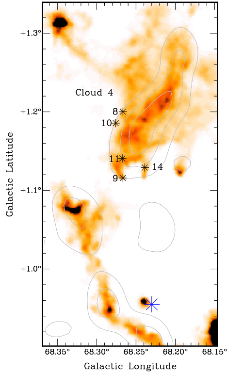
Figure 12. 250 \mu\text{m} emission distribution in the area of the molecular Cloud 4. The five WISE sources located on to this cloud are indicated with asterisks and with their corresponding numbers (see Table 4). Grey contours are from 0.4 to 1.6 K with a step of 0.4 K and correspond to the averaged CO emission between -7.18 and -0.7 \text{km s}^{-1} . The location of WR 130 is indicated by the blue asterisk.
