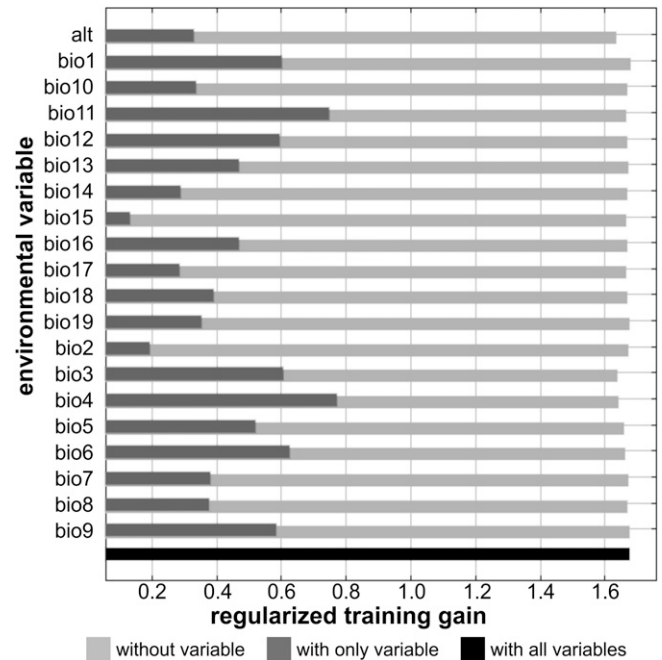
Figure 5. Jackknife test of training gain for the MaxEnt model. Abbreviations: alt , elevation, bio1 through bio19 , bioclimatic variables (Table 2).
