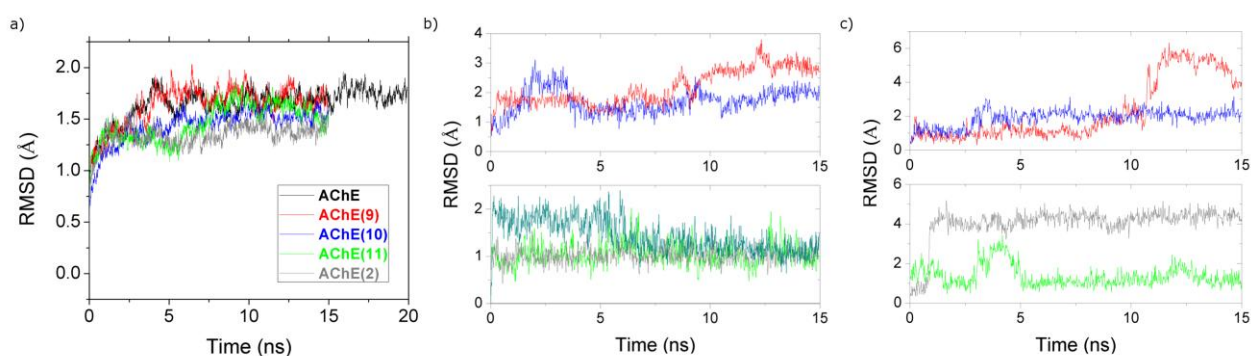
Figure 3. a) Evolution of the RMSD of the backbone of the protein for the MD runs of AChE and AChE with compounds 9-11 and 2 at the AS. b) Evolution of the RMSD of the ligands at the AS, without considering the hydrogen atoms. c) Evolution of the RMSD of the ligands at the PAS, without considering the hydrogen atoms. The same color was employed in all the graphics for representing the properties of each MD run. AChE (■), AChE-9 (■), AChE-10 (■), AChE-11a (■), AChE-11b (■) and AChE-2 (■).
