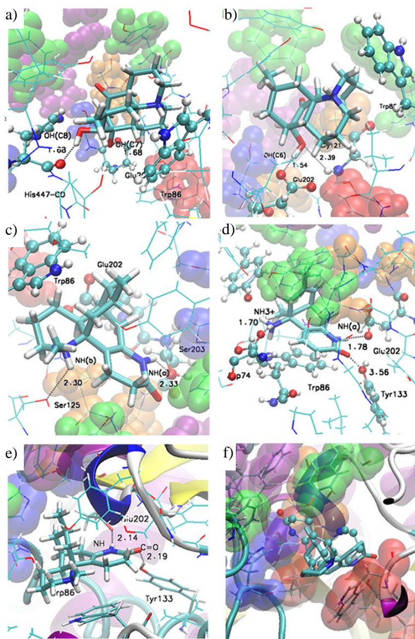
Figure 5. 3-D plot of the final geometries obtained after 15 ns of MD simulation. For the complexes: a) AChE-9, b) AChE-10, c) AChE-11a d) AChE-2, e) AChE-11b (similar to 2). f) Comparison of the geometries: 11a (represented with balls and sticks) and 11b (represented with bold sticks). The hydrogen bonds are represented by black dotted lines.
