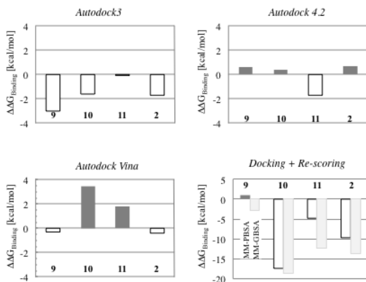
Figure 2. Preference for the binding at the AS and PAS sites obtained with different procedures. The histograms represent the difference in binding free energies ( \Delta\Delta G_{\text{Binding}} = \Delta G_{\text{Binding AS}} - \Delta G_{\text{Binding PAS}} ). Light bars show a preference for the AS while dark ones show a predilection for the PAS.
