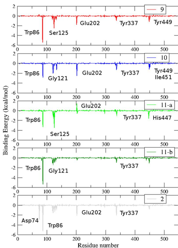
Figure 4. Per-residue contributions to the binding energy calculated with MM-GBSA from the MD simulations of 9-11, 2 at the AS site. AChE- 9 (■), AChE- 10 (■), AChE- 11a (■), AChE- 11b (■) and AChE- 2 (■).
