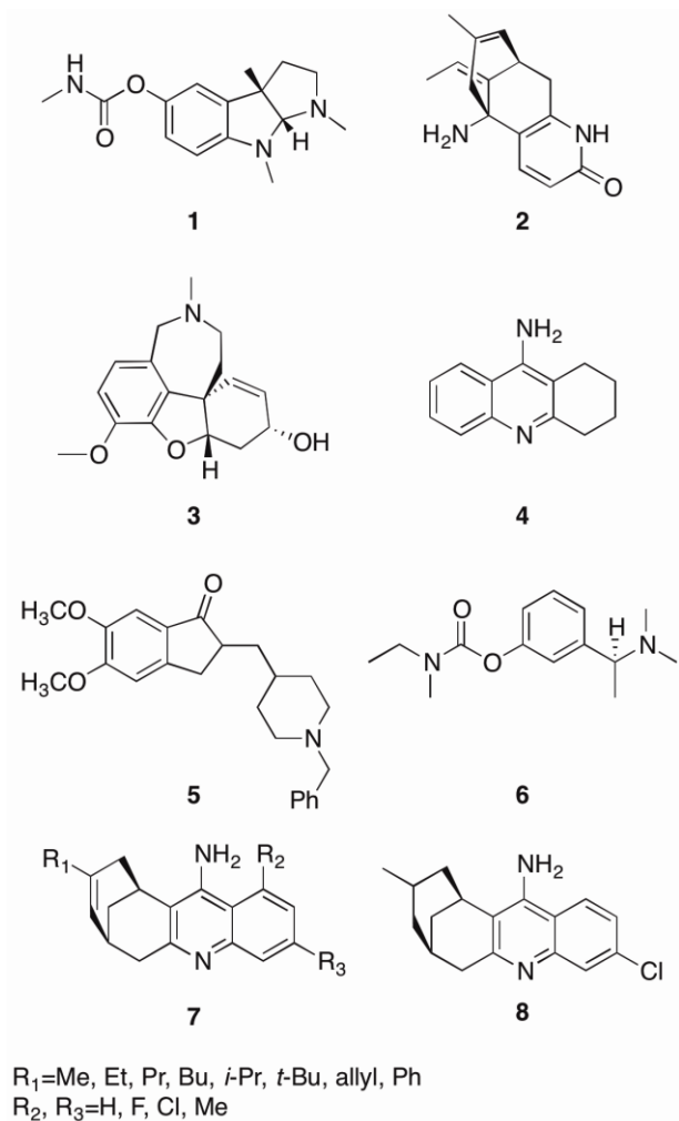
Scheme 1. AChE inhibitors
