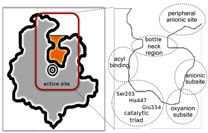
Figure 1. Schematic description of the active site of the AChE and the corresponding subsites.
