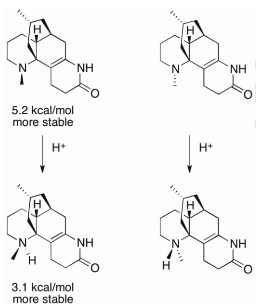
Scheme 3. Different conformers of 11 according to the position of the \beta -N-methyl group.
