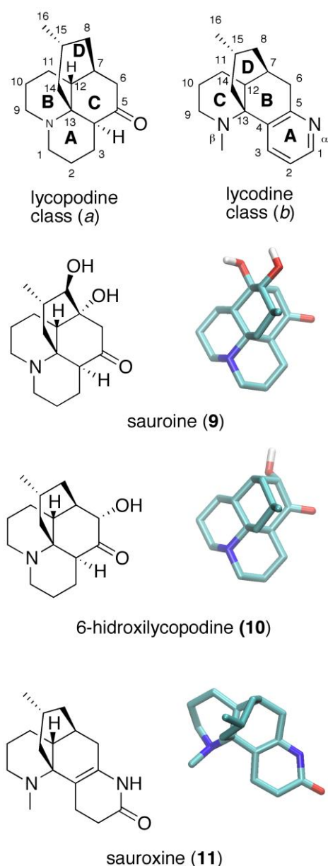
Scheme 2. Proposed AChEI extracted from Huperzia saururus
