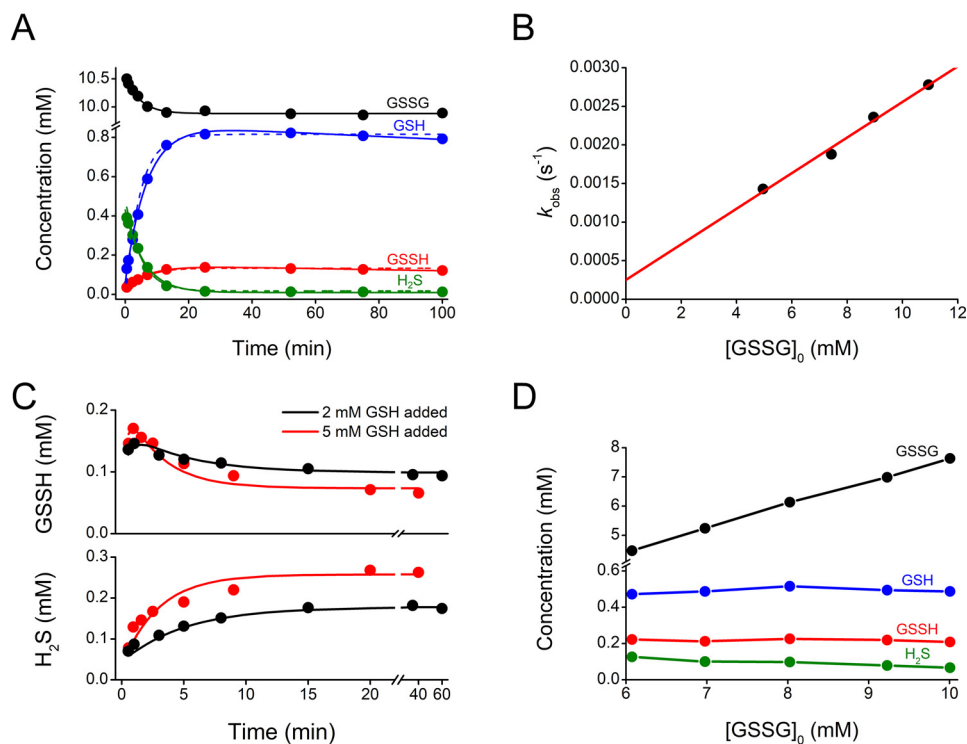
Figure 2. Kinetics and thermodynamics of the reaction of GSSG and H 2 S to give GSH and GSSH. A , time courses of the reaction between GSSG (11 mM) and H 2 S (0.5 mM) in phosphate buffer (0.1 M, pH 7.4, 25 ± 1 °C). Solid lines represent the fitted single exponential or exponential plus linear functions. The rate constants of a model consisting of Reactions 1 and 2 were estimated with COPASI using four independent experiments, obtaining k_{1,pH} = 0.33 \pm 0.01 , k_{-1,pH} = 0.51 \pm 0.08 , k_{2,pH} = 1.6 \pm 0.3 , and k_{-2,pH} = 9 \pm 2 \text{ M}^{-1} \text{ s}^{-1} . Dashed lines represent simulated time courses for a representative experiment. B , exponential rate constants ( k_{\text{obs}} ) of H 2 S decay versus initial GSSG. The k_{1,pH} obtained from the fit of four independent experiments was 0.23 \pm 0.02 \text{ M}^{-1} \text{ s}^{-1} (pH 7.46 ± 0.01, 24 °C). C , mixtures of GSSG (5 mM) and H 2 S (0.5 mM), preincubated for 1 h in the mentioned buffer, were exposed to 2–12.5 mM GSH, and the reactions were followed by derivatization and HPLC (pH 7.28 ± 0.05, 25 °C). Using eight independent experiments, COPASI simulations in which k_{1,pH} was fixed to 0.23 \text{ M}^{-1} \text{ s}^{-1} , and initial concentrations of GSSG, GSSH, and H 2 S were 3.7 mM, 90 μM, and 50 μM, respectively, according to HPLC quantification, yielded k_{-1,pH} = 1.11 \pm 0.06 , k_{2,pH} = 2.3 \pm 0.5 , k_{-2,pH} = 3.1 \pm 0.4 \text{ M}^{-1} \text{ s}^{-1} , and [\text{GSSG}]_0 = 0.27 \pm 0.01 \text{ mM} . Solid lines represent simulated time courses for two representative experiments. D , equilibrium concentrations. GSSG (6–10 mM) and H 2 S (0.5 mM) were incubated in the mentioned buffer under shaking. After 2 h, 4 mM mBrB was added and the GSSH-containing mixtures were analyzed by HPLC. The apparent equilibrium constant of Reaction 1 obtained from six independent determinations was 0.194 \pm 0.005 (mean ± S.D., pH 7.4, 25 °C).
