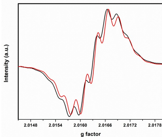
Figure 4. Comparison between the room temperature EPR spectra of degassed TEMPOL dissolved in ethylene glycol. The black and red lines is the spectra obtained in the absence and presence of Au/ZnO nanostructures.
