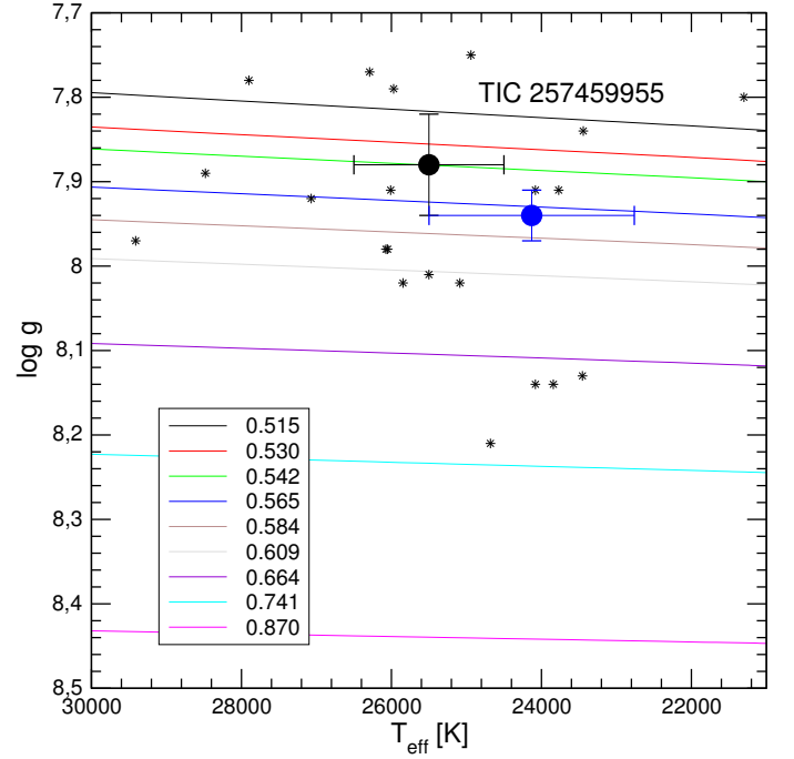
Fig. 5. Location of the known DBV stars on the T_{\text{eff}}\text{--}\log g diagram (black star symbols) according to the compilation by Córscico et al. (2019). The DB white dwarf evolutionary tracks are depicted with different colors according to the stellar mass. Stellar masses are in solar units. The location of TIC 257459955 as given by spectroscopy according to Voss et al. (2007) and Rolland et al. (2018) are highlighted with black and blue circles and error bars. The stellar mass derived from linear interpolation results M_\star = 0.542^{+0.028}_{-0.025} M_\odot using the data from Voss et al. (2007), and M_\star = 0.570^{+0.009}_{-0.011} M_\odot employing the data from Rolland et al. (2018).
