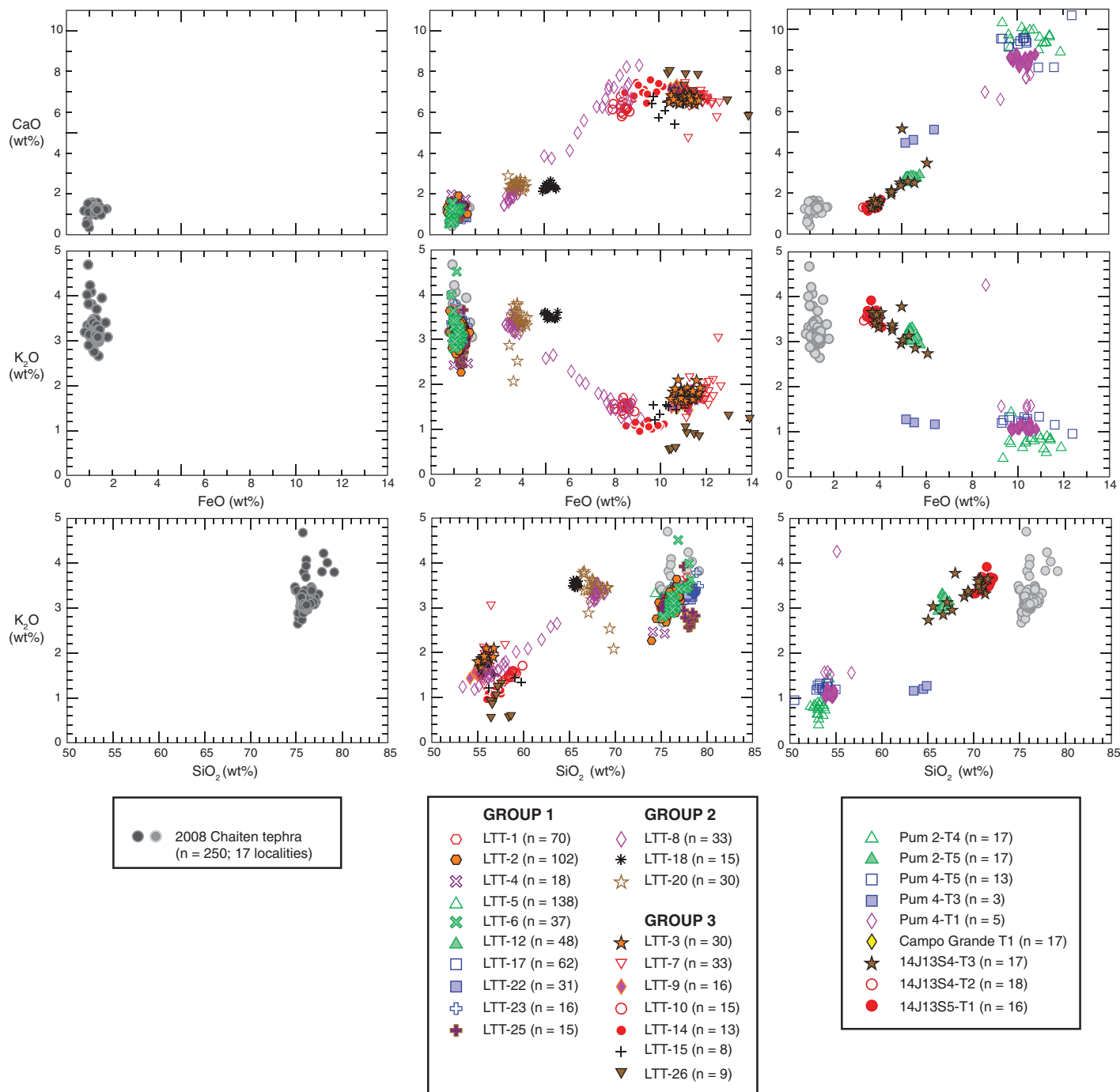
Figure 2. CaO and K 2 O versus FeO t , and K 2 O versus SiO 2 (wt%) for glass shards from tephra layers preserved in Lago Teo (southern Chile) sediment core. Lago Teo tephra (LTT) are divided into three broad compositional groupings based on glass shard major element geochemistry. In order to identify potential eruptive sources, these groupings are compared with glass shard analyses from the A.D. 2008 Volcán Chaitén eruption (Alloway and Villarosa, this study), as well as equivalent-aged proximal Michinmahuida volcanic complex-sourced tephra preserved in the adjacent andic soil-forming environment (see Fig. DR1 [see footnote 1]).
